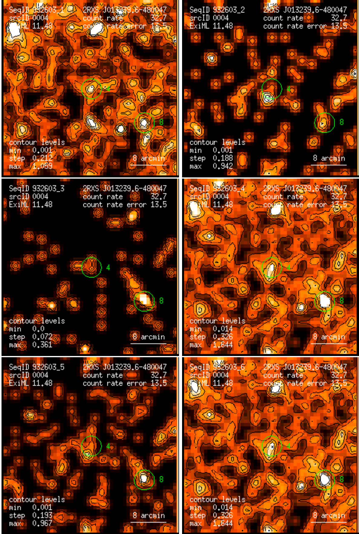
Figure 4: RASS 932603: detection 0004: band rate images, Gaussian filter: (1) PSPC channels 11 – 41, (2) 52 – 90, (3) 91 – 201, (4) 11 – 235, (5) 52 – 201, (6) 11 – 201. Broad band rates in counts/ks. Band rate contour levels in counts/ks/arcmin 2 .
