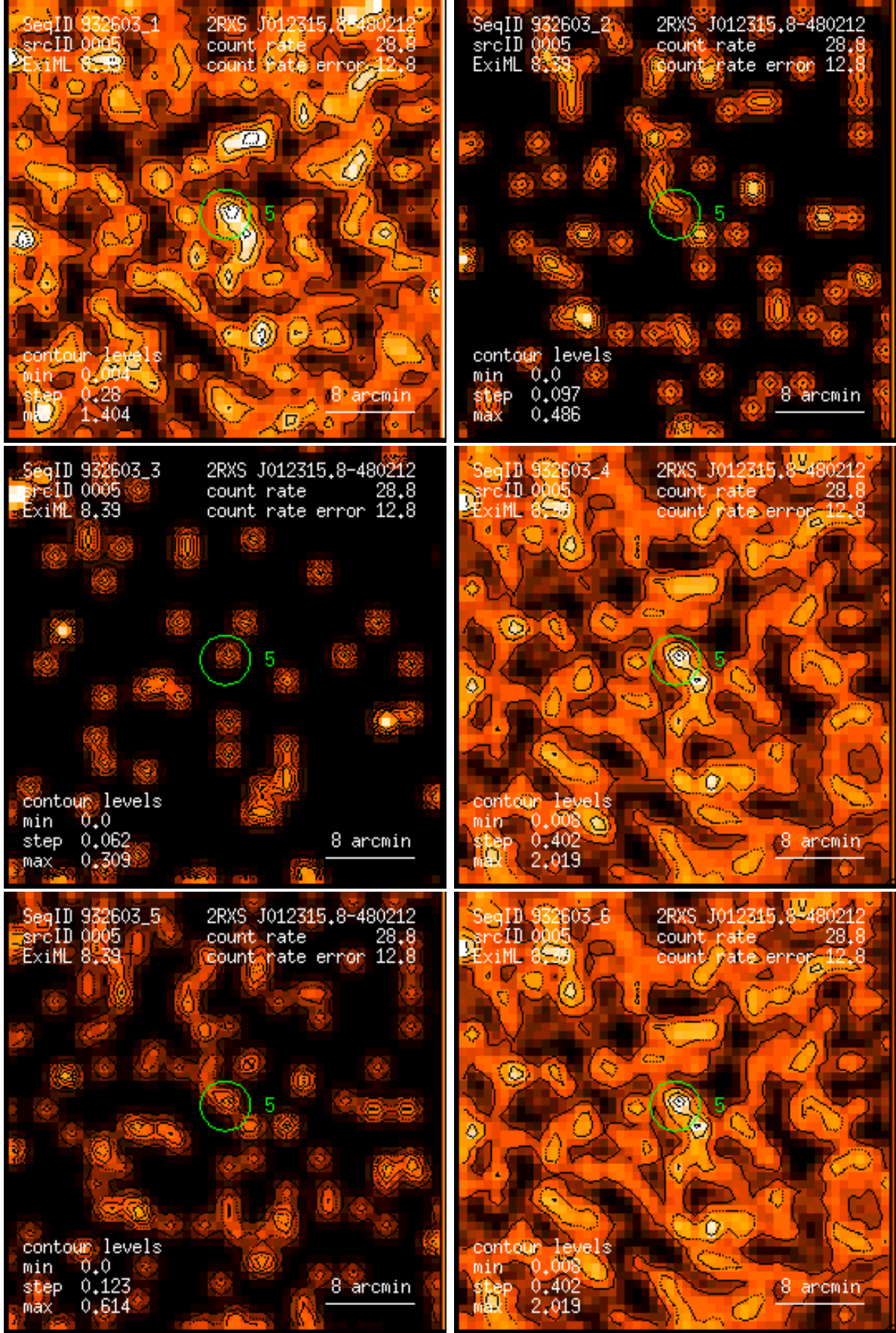
Figure 5: RASS 932603: detection 0005: band rate images, Gaussian filter: (1) PSPC channels 11 – 41, (2) 52 – 90, (3) 91 – 201, (4) 11 – 235, (5) 52 – 201, (6) 11 – 201. Broad band rates in counts/ks. Band rate contour levels in counts/ks/arcmin 2 .
