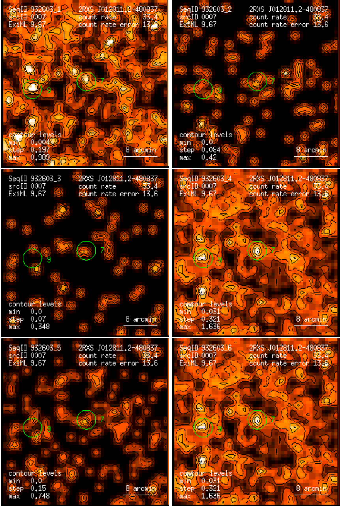
Figure 7: RASS 932603: detection 0007: band rate images, Gaussian filter: (1) PSPC channels 11 – 41, (2) 52 – 90, (3) 91 – 201, (4) 11 – 235, (5) 52 – 201, (6) 11 – 201. Broad band rates in counts/ks. Band rate contour levels in counts/ks/arcmin 2 .
