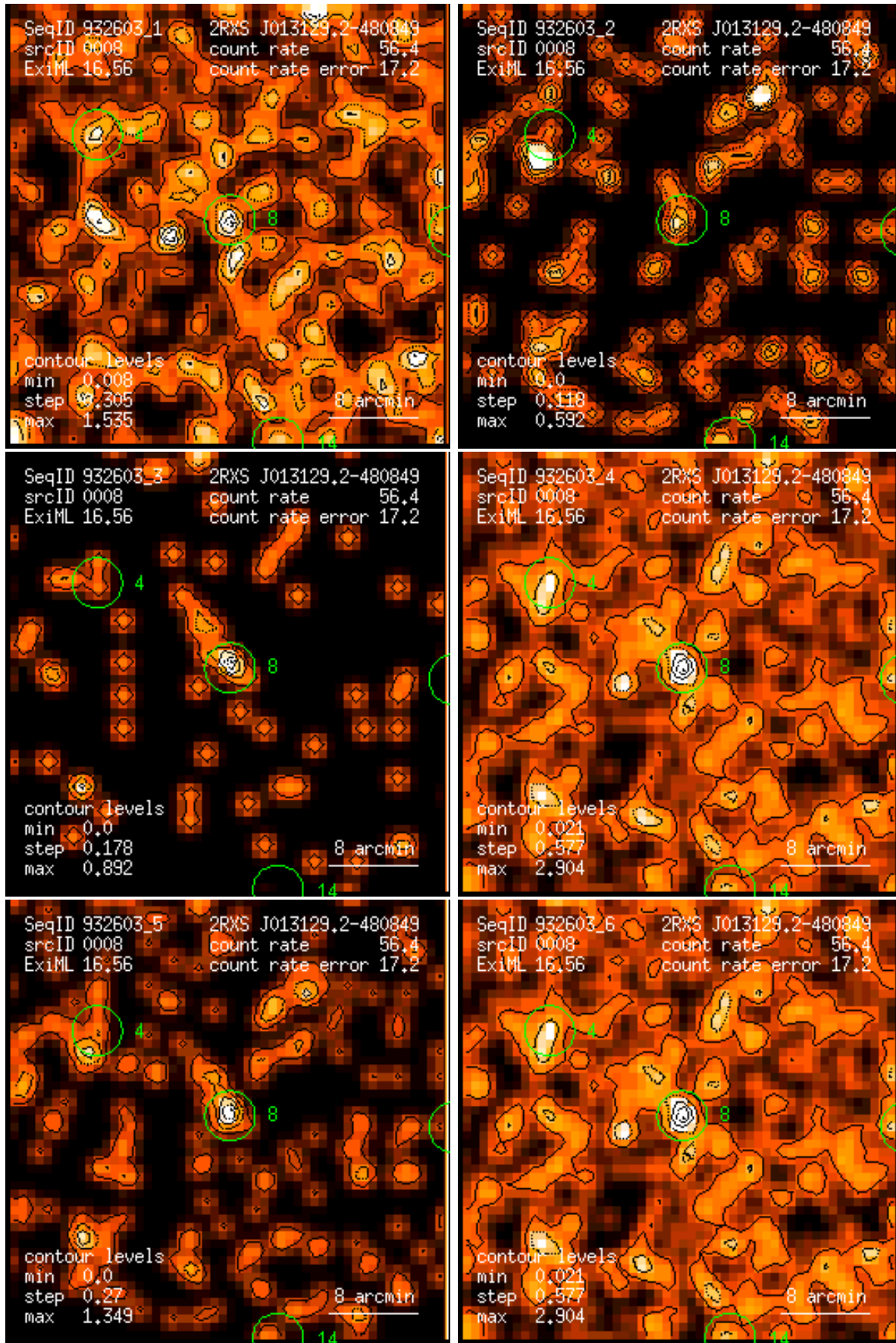
Figure 8: RASS 932603: detection 0008: band rate images, Gaussian filter: (1) PSPC channels 11 – 41, (2) 52 – 90, (3) 91 – 201, (4) 11 – 235, (5) 52 – 201, (6) 11 – 201. Broad band rates in counts/ks. Band rate contour levels in counts/ks/arcmin 2 .
