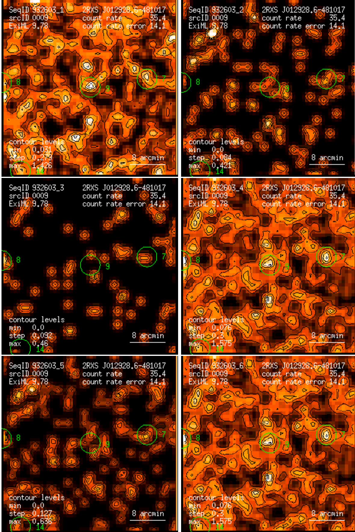
Figure 9: RASS 932603: detection 0009: band rate images, Gaussian filter: (1) PSPC channels 11 – 41, (2) 52 – 90, (3) 91 – 201, (4) 11 – 235, (5) 52 – 201, (6) 11 – 201. Broad band rates in counts/ks. Band rate contour levels in counts/ks/arcmin 2 .
