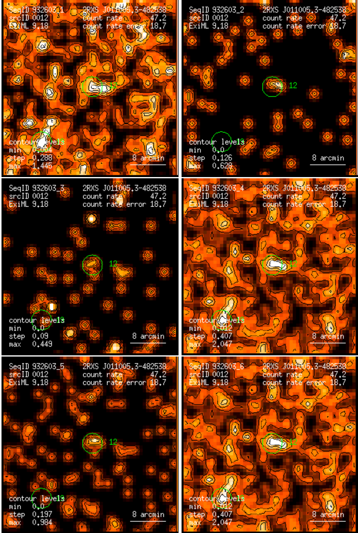
Figure 12: RASS 932603: detection 0012: band rate images, Gaussian filter: (1) PSPC channels 11 – 41, (2) 52 – 90, (3) 91 – 201, (4) 11 – 235, (5) 52 – 201, (6) 11 – 201. Broad band rates in counts/ks. Band rate contour levels in counts/ks/arcmin 2 .
