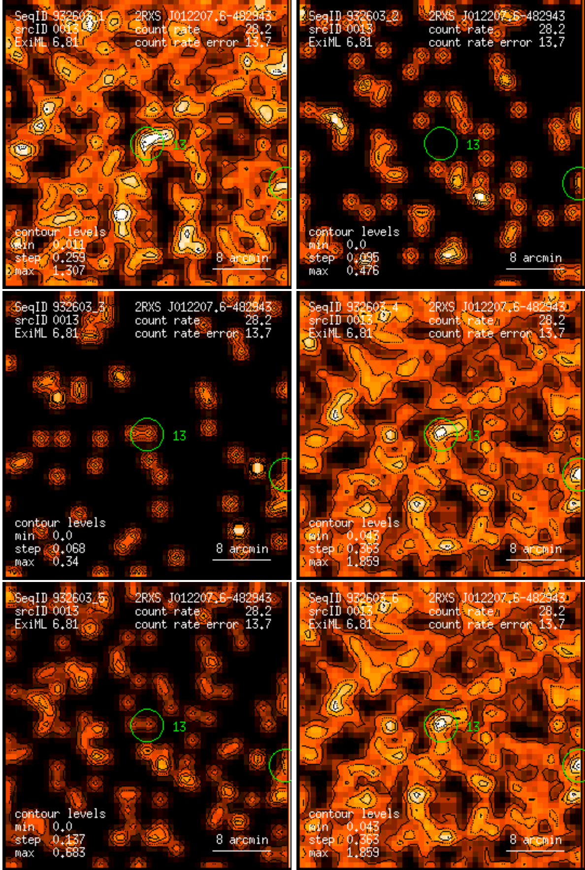
Figure 13: RASS 932603: detection 0013: band rate images, Gaussian filter: (1) PSPC channels 11 – 41, (2) 52 – 90, (3) 91 – 201, (4) 11 – 235, (5) 52 – 201, (6) 11 – 201. Broad band rates in counts/ks. Band rate contour levels in counts/ks/arcmin 2 .
