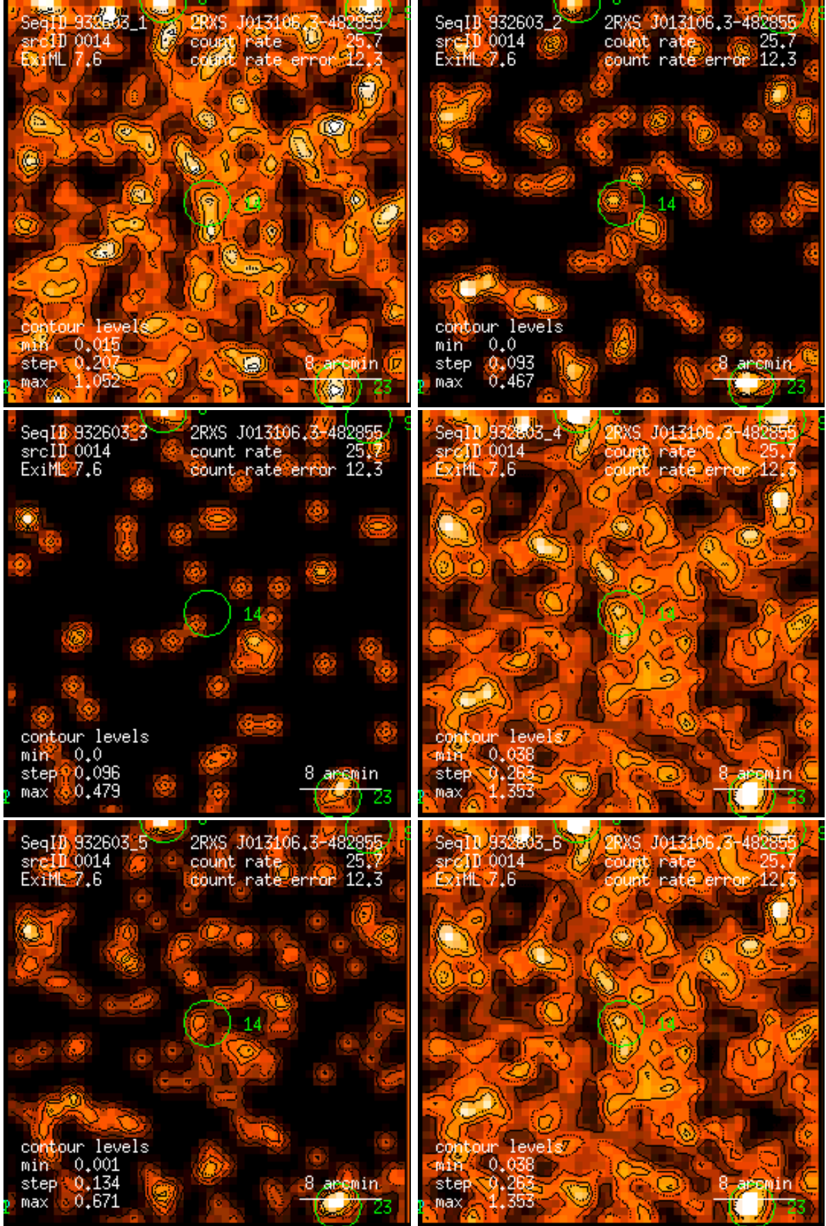
Figure 14: RASS 932603: detection 0014: band rate images, Gaussian filter: (1) PSPC channels 11 – 41, (2) 52 – 90, (3) 91 – 201, (4) 11 – 235, (5) 52 – 201, (6) 11 – 201. Broad band rates in counts/ks. Band rate contour levels in counts/ks/arcmin 2 .
