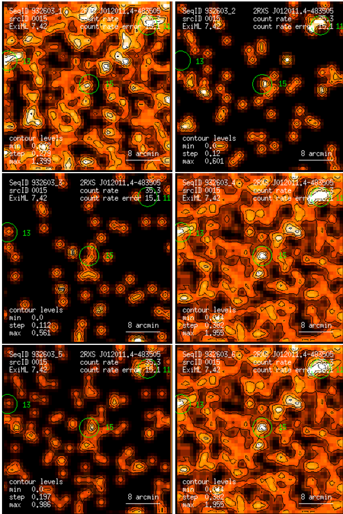
Figure 15: RASS 932603: detection 0015: band rate images, Gaussian filter: (1) PSPC channels 11 – 41, (2) 52 – 90, (3) 91 – 201, (4) 11 – 235, (5) 52 – 201, (6) 11 – 201. Broad band rates in counts/ks. Band rate contour levels in counts/ks/arcmin 2 .
