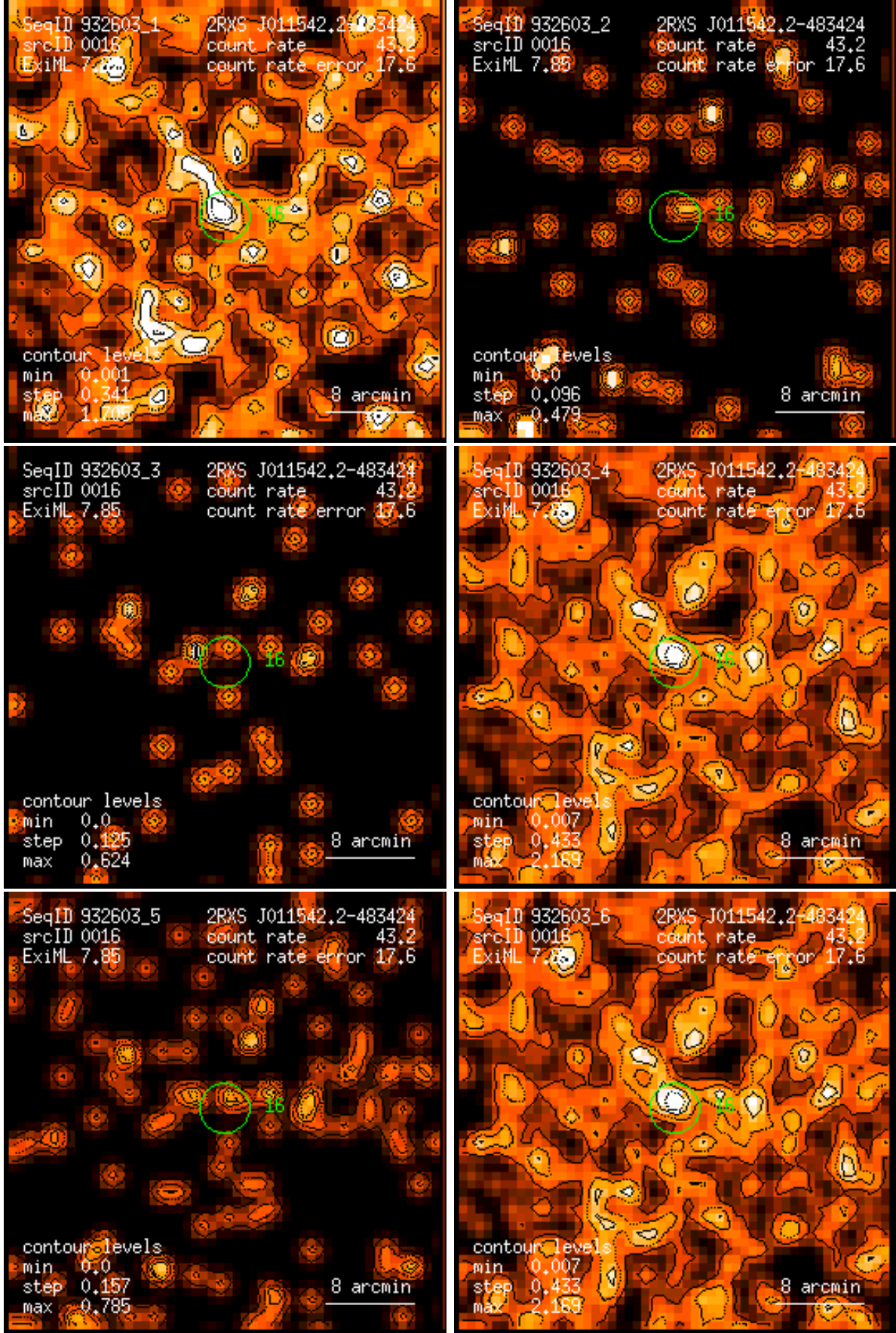
Figure 16: RASS 932603: detection 0016: band rate images, Gaussian filter: (1) PSPC channels 11 – 41, (2) 52 – 90, (3) 91 – 201, (4) 11 – 235, (5) 52 – 201, (6) 11 – 201. Broad band rates in counts/ks. Band rate contour levels in counts/ks/arcmin 2 .
