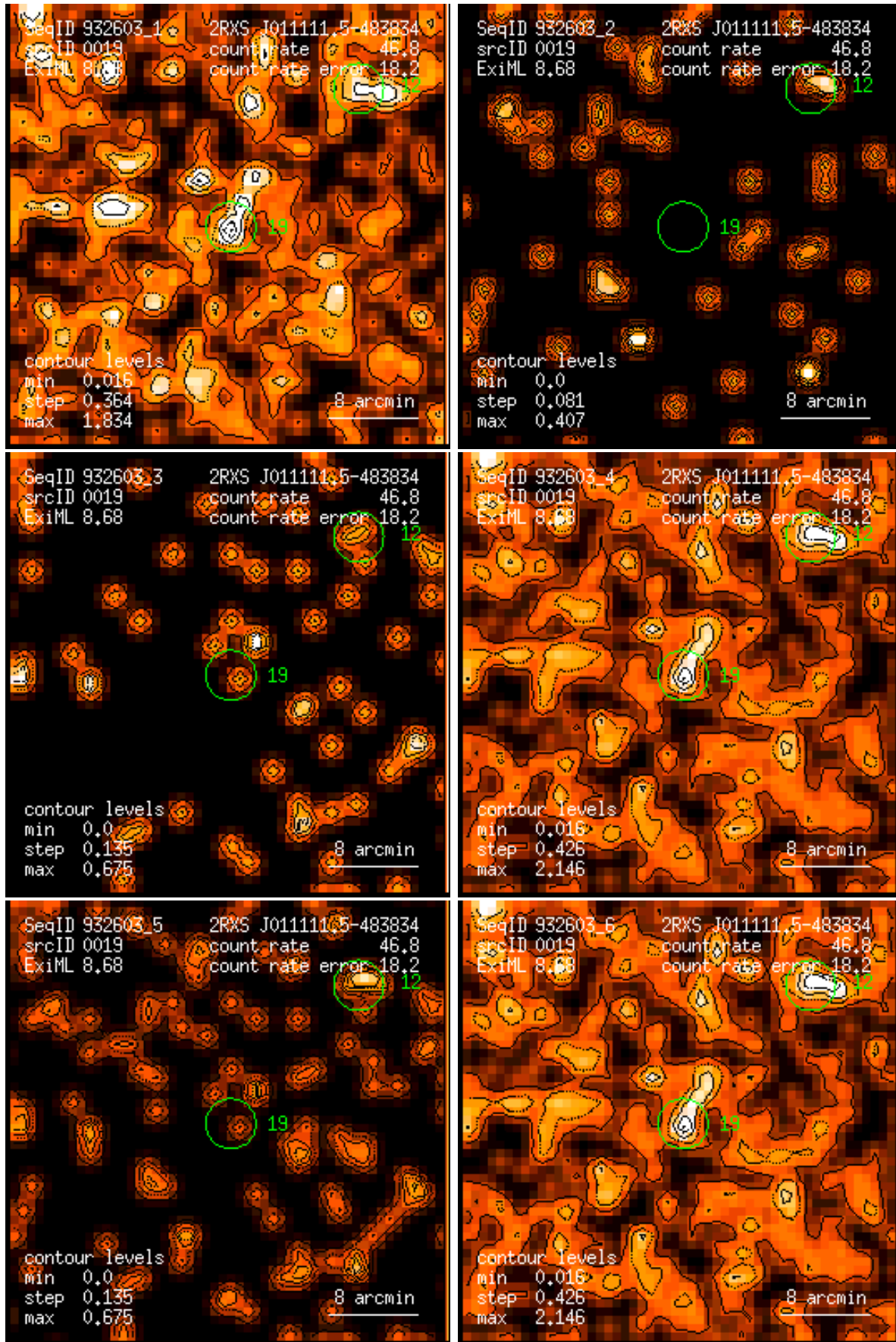
Figure 19: RASS 932603: detection 0019: band rate images, Gaussian filter: (1) PSPC channels 11 – 41, (2) 52 – 90, (3) 91 – 201, (4) 11 – 235, (5) 52 – 201, (6) 11 – 201. Broad band rates in counts/ks. Band rate contour levels in counts/ks/arcmin 2 .
