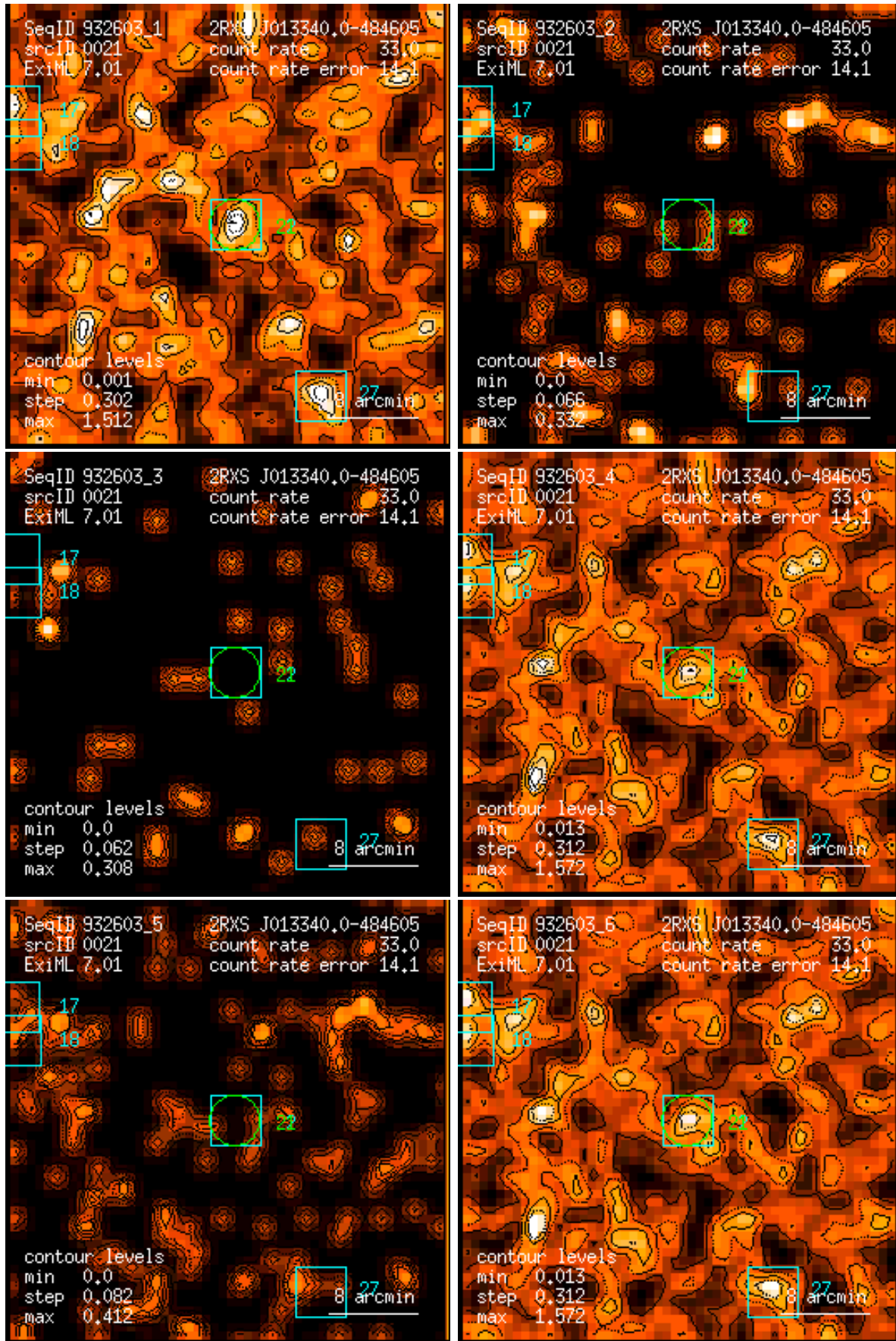
Figure 21: RASS 932603: detection 0021: band rate images, Gaussian filter: (1) PSPC channels 11 – 41, (2) 52 – 90, (3) 91 – 201, (4) 11 – 235, (5) 52 – 201, (6) 11 – 201. Broad band rates in counts/ks. Band rate contour levels in counts/ks/arcmin 2 .
