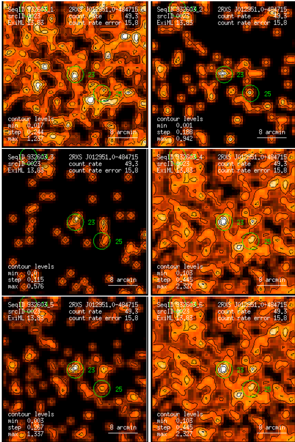
Figure 23: RASS 932603: detection 0023: band rate images, Gaussian filter: (1) PSPC channels 11 – 41, (2) 52 – 90, (3) 91 – 201, (4) 11 – 235, (5) 52 – 201, (6) 11 – 201. Broad band rates in counts/ks. Band rate contour levels in counts/ks/arcmin 2 .
