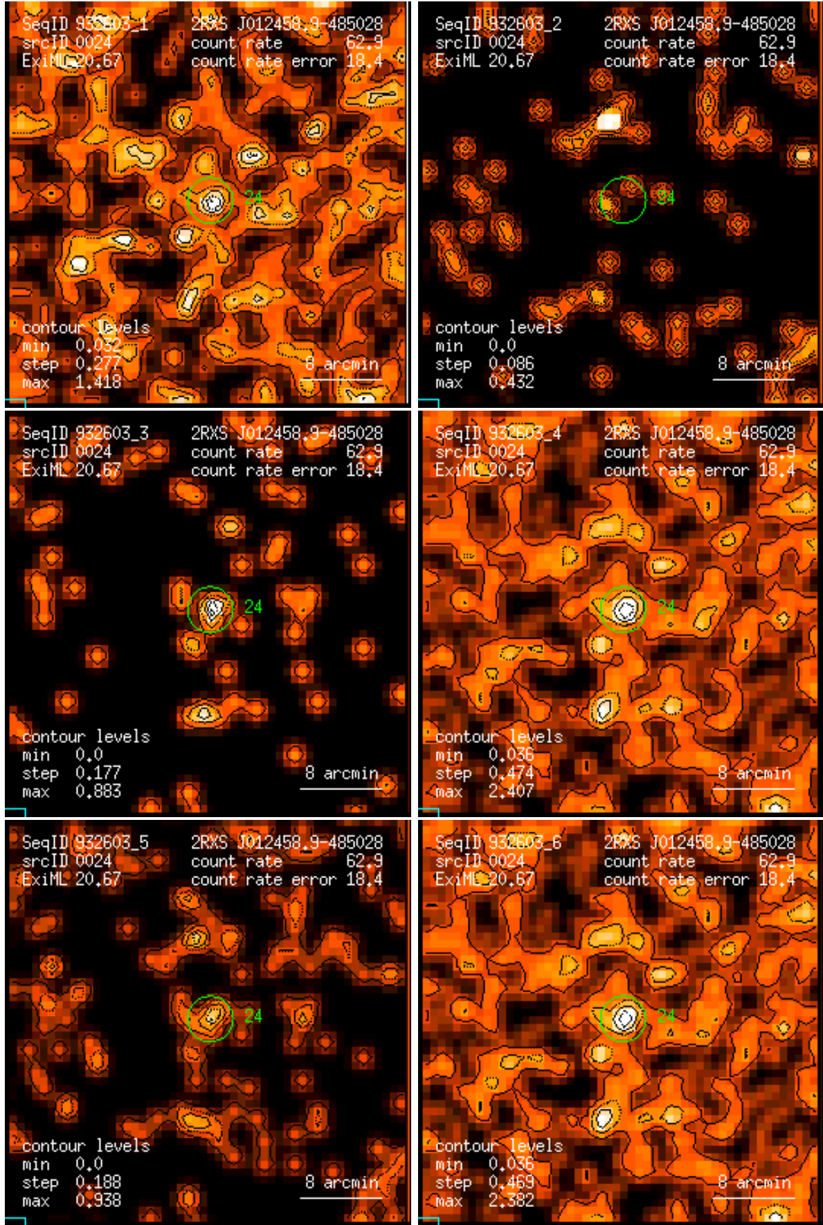
Figure 24: RASS 932603: detection 0024: band rate images, Gaussian filter: (1) PSPC channels 11 – 41, (2) 52 – 90, (3) 91 – 201, (4) 11 – 235, (5) 52 – 201, (6) 11 – 201. Broad band rates in counts/ks. Band rate contour levels in counts/ks/arcmin 2 .
