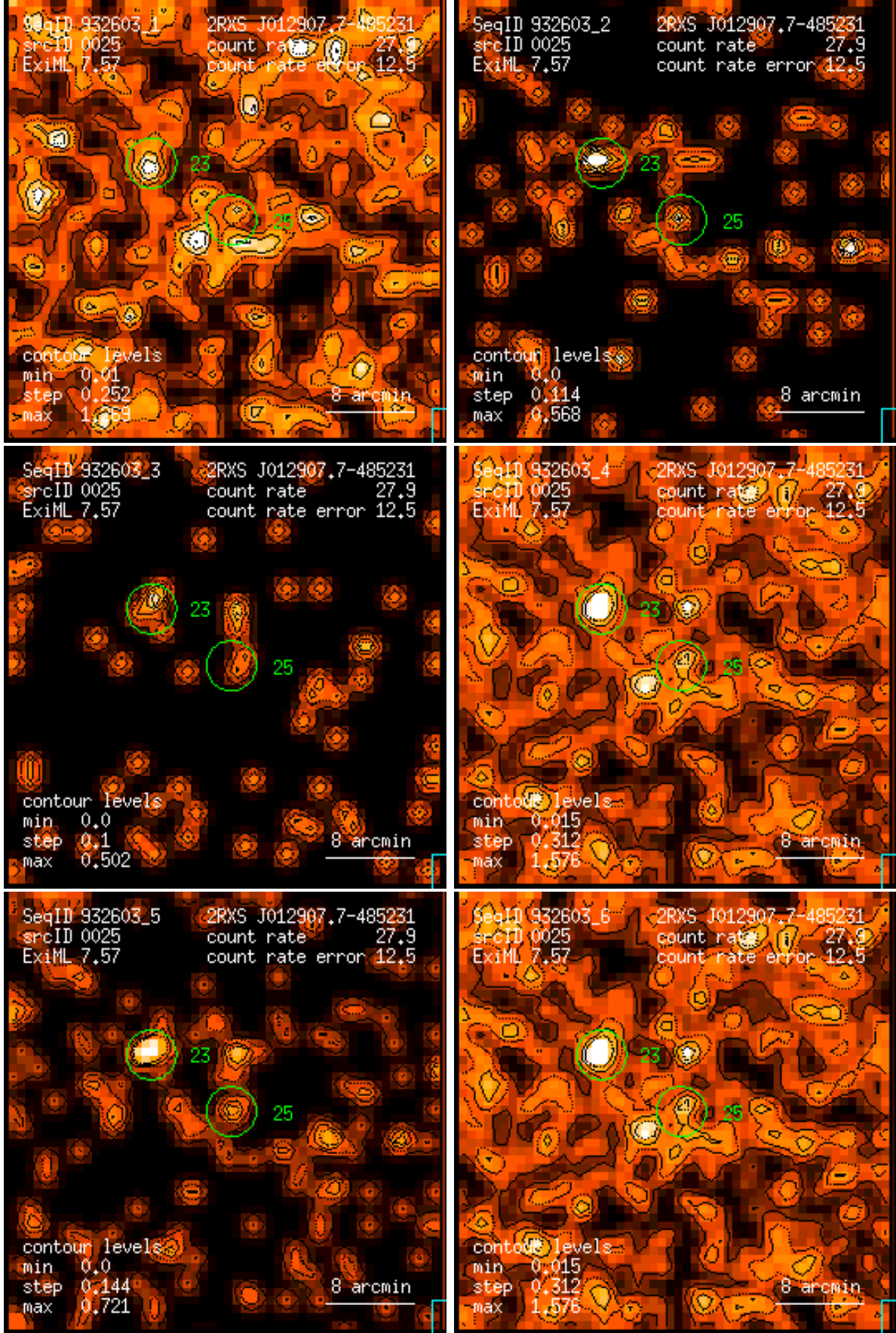
Figure 25: RASS 932603: detection 0025: band rate images, Gaussian filter: (1) PSPC channels 11 – 41, (2) 52 – 90, (3) 91 – 201, (4) 11 – 235, (5) 52 – 201, (6) 11 – 201. Broad band rates in counts/ks. Band rate contour levels in counts/ks/arcmin 2 .
