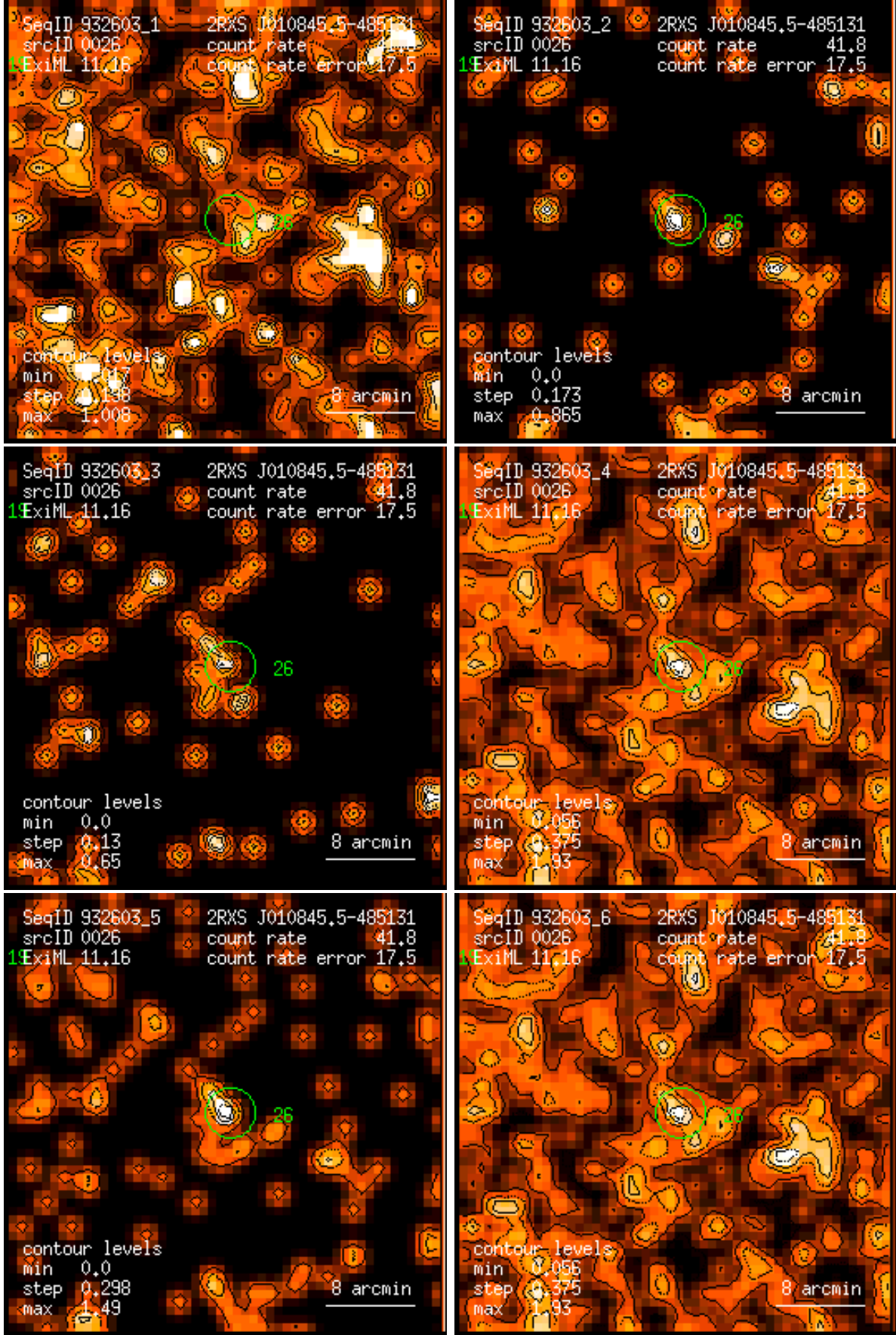
Figure 26: RASS 932603: detection 0026: band rate images, Gaussian filter: (1) PSPC channels 11 – 41, (2) 52 – 90, (3) 91 – 201, (4) 11 – 235, (5) 52 – 201, (6) 11 – 201. Broad band rates in counts/ks. Band rate contour levels in counts/ks/arcmin 2 .
