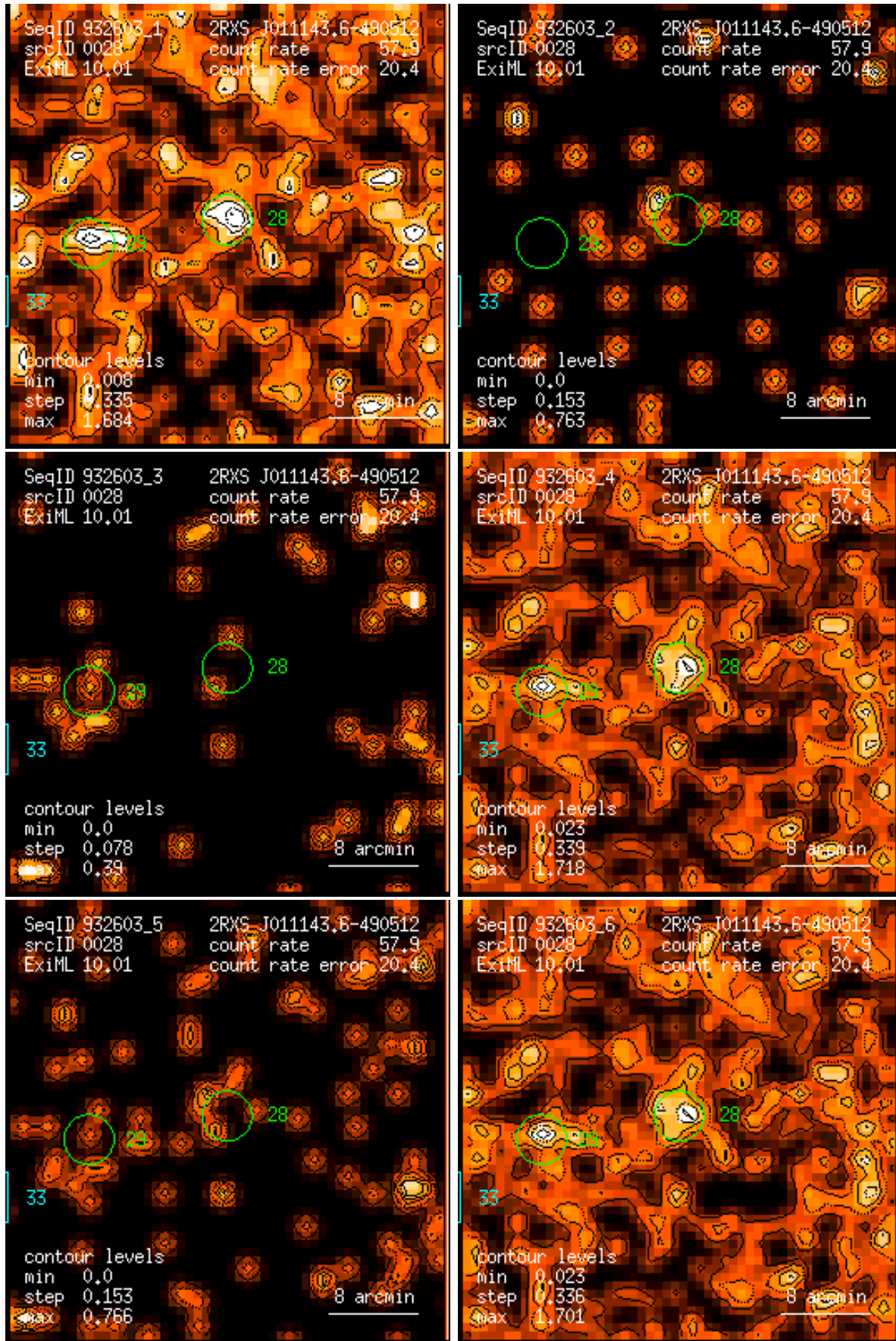
Figure 28: RASS 932603: detection 0028: band rate images, Gaussian filter: (1) PSPC channels 11 – 41, (2) 52 – 90, (3) 91 – 201, (4) 11 – 235, (5) 52 – 201, (6) 11 – 201. Broad band rates in counts/ks. Band rate contour levels in counts/ks/arcmin 2 .
