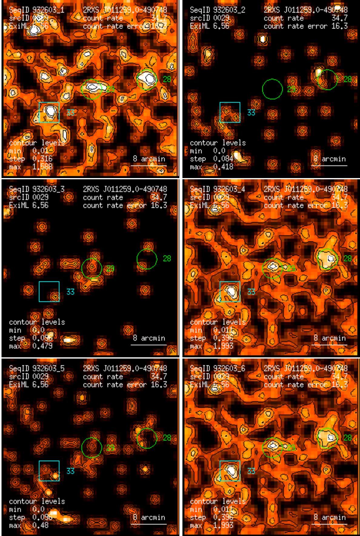
Figure 29: RASS 932603: detection 0029: band rate images, Gaussian filter: (1) PSPC channels 11 – 41, (2) 52 – 90, (3) 91 – 201, (4) 11 – 235, (5) 52 – 201, (6) 11 – 201. Broad band rates in counts/ks. Band rate contour levels in counts/ks/arcmin 2 .
