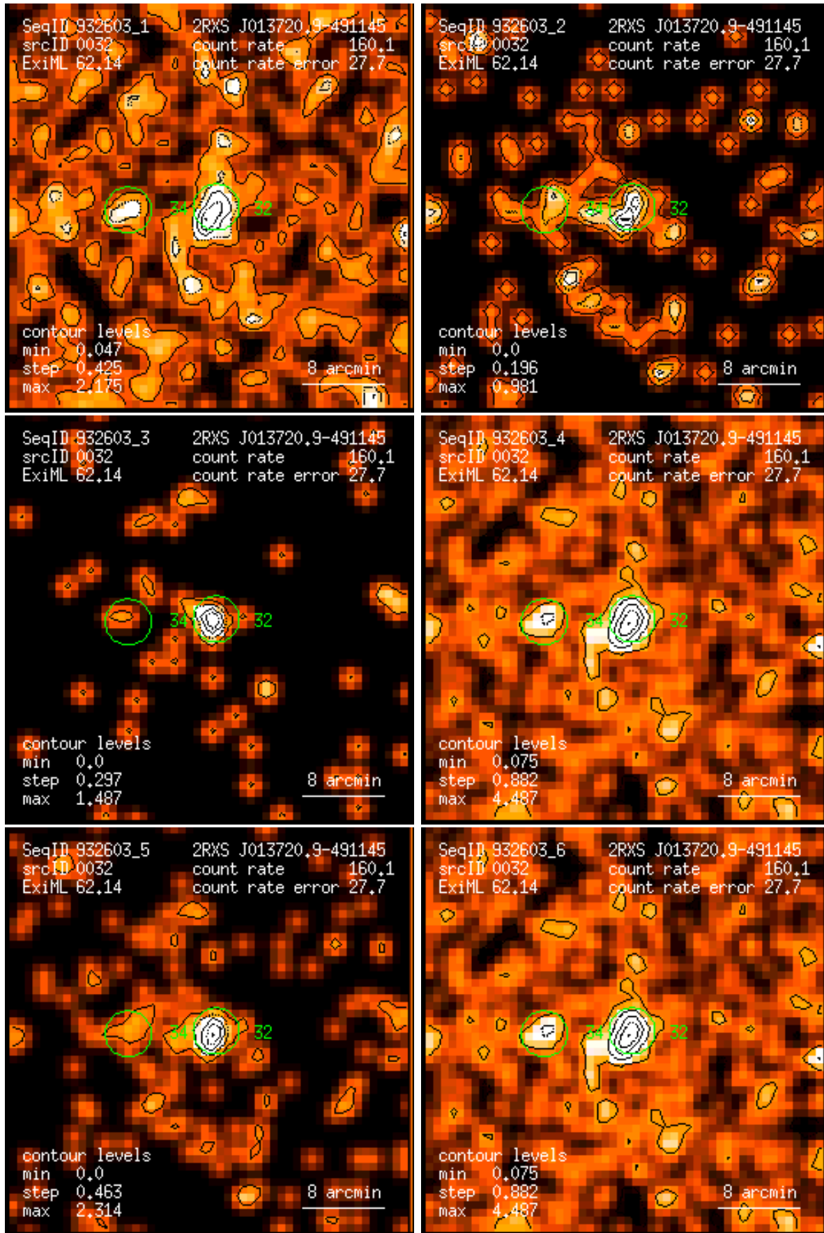
Figure 32: RASS 932603: detection 0032: band rate images, Gaussian filter: (1) PSPC channels 11 – 41, (2) 52 – 90, (3) 91 – 201, (4) 11 – 235, (5) 52 – 201, (6) 11 – 201. Broad band rates in counts/ks. Band rate contour levels in counts/ks/arcmin 2 .
