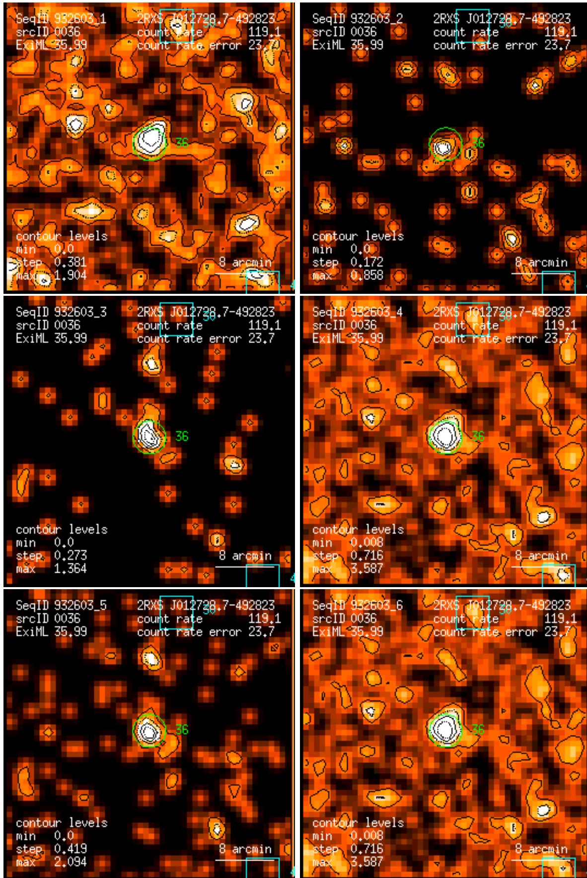
Figure 36: RASS 932603: detection 0036: band rate images, Gaussian filter: (1) PSPC channels 11 – 41, (2) 52 – 90, (3) 91 – 201, (4) 11 – 235, (5) 52 – 201, (6) 11 – 201. Broad band rates in counts/ks. Band rate contour levels in counts/ks/arcmin 2 .
