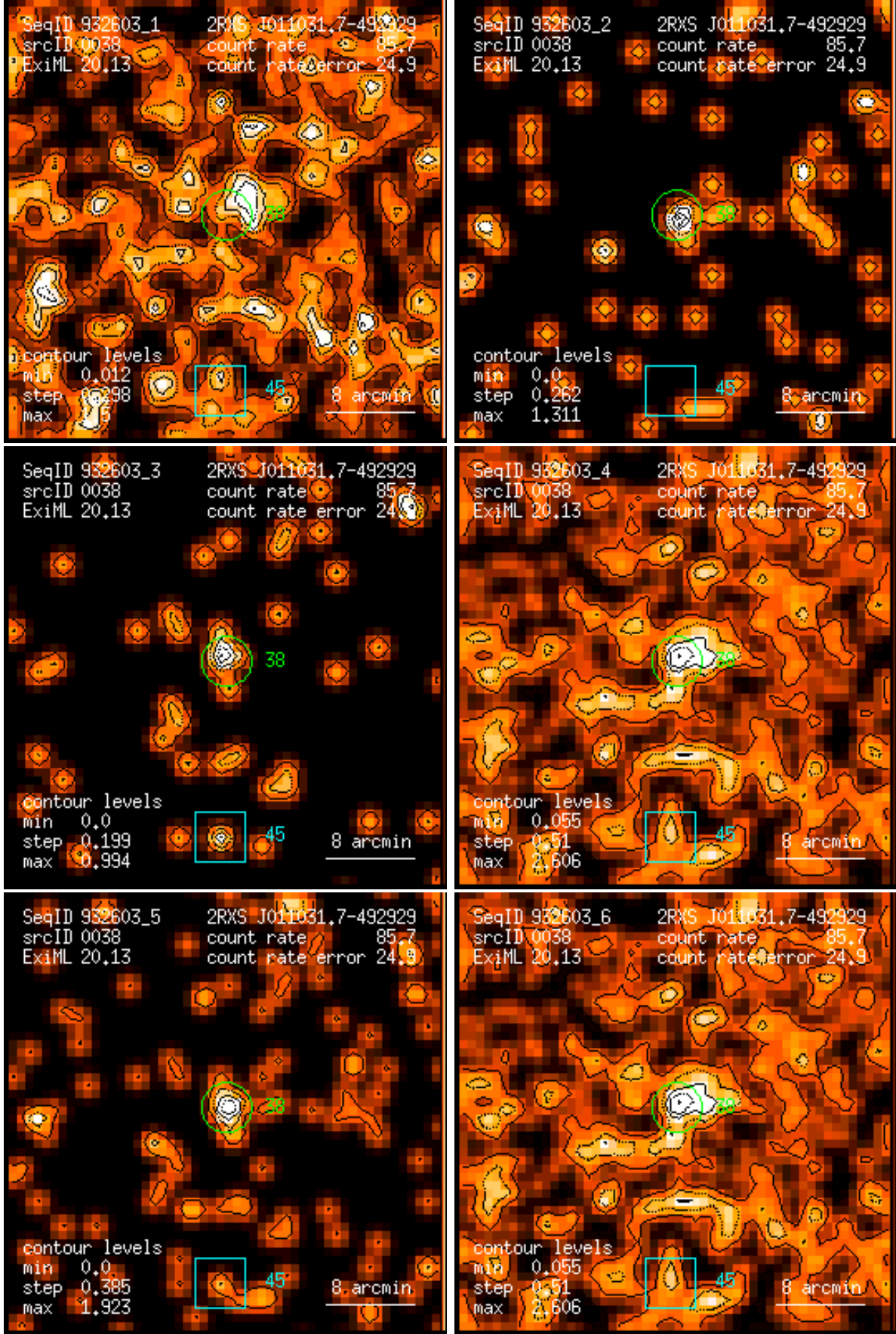
Figure 38: RASS 932603: detection 0038: band rate images, Gaussian filter: (1) PSPC channels 11 – 41, (2) 52 – 90, (3) 91 – 201, (4) 11 – 235, (5) 52 – 201, (6) 11 – 201. Broad band rates in counts/ks. Band rate contour levels in counts/ks/arcmin 2 .
