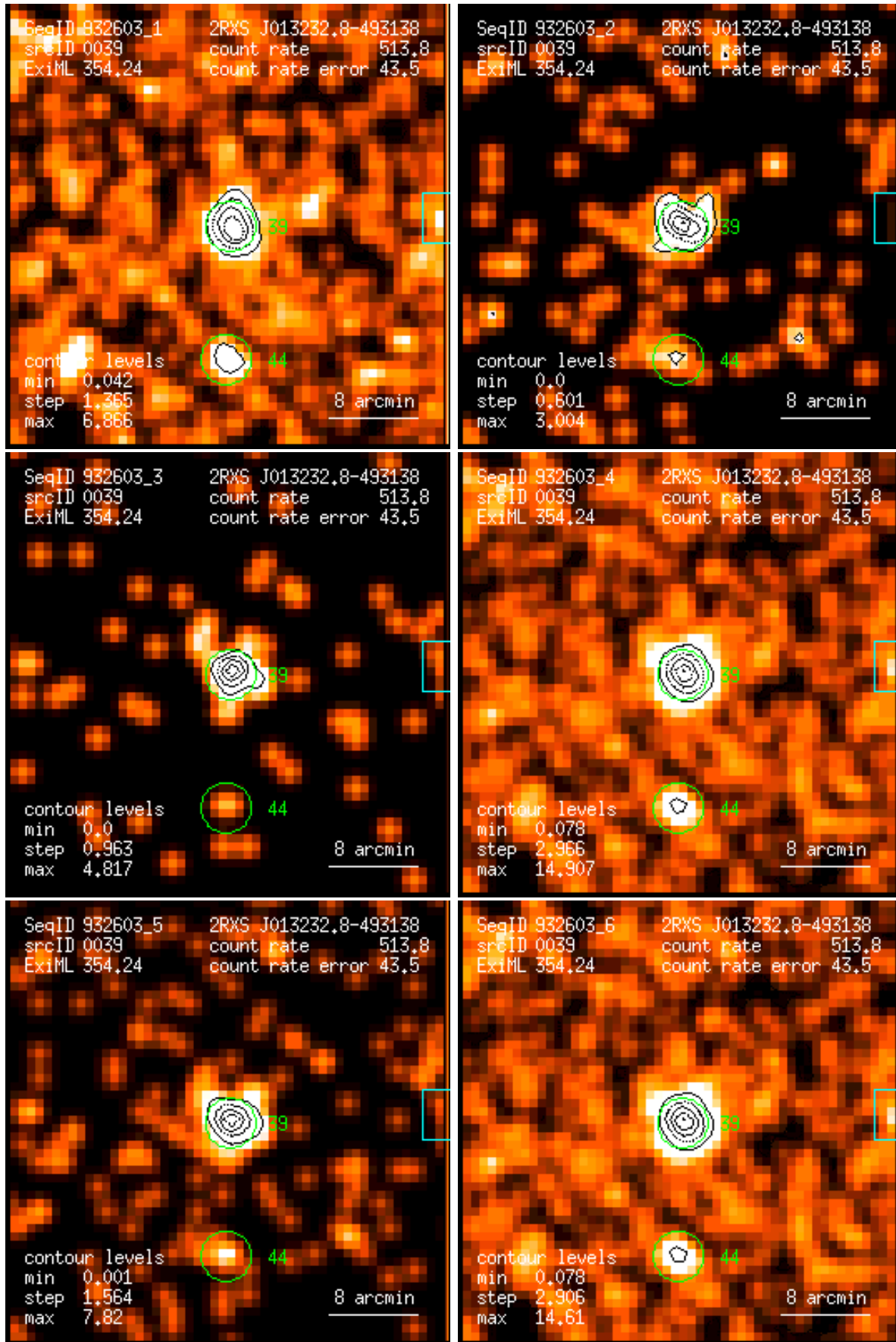
Figure 39: RASS 932603: detection 0039: band rate images, Gaussian filter: (1) PSPC channels 11 – 41, (2) 52 – 90, (3) 91 – 201, (4) 11 – 235, (5) 52 – 201, (6) 11 – 201. Broad band rates in counts/ks. Band rate contour levels in counts/ks/arcmin 2 .
