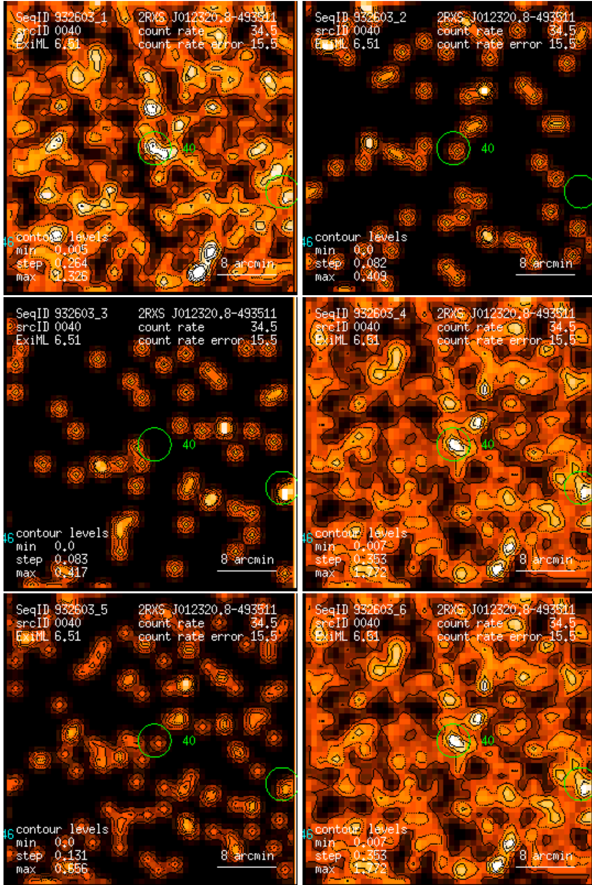
Figure 40: RASS 932603: detection 0040: band rate images, Gaussian filter: (1) PSPC channels 11 – 41, (2) 52 – 90, (3) 91 – 201, (4) 11 – 235, (5) 52 – 201, (6) 11 – 201. Broad band rates in counts/ks. Band rate contour levels in counts/ks/arcmin 2 .
