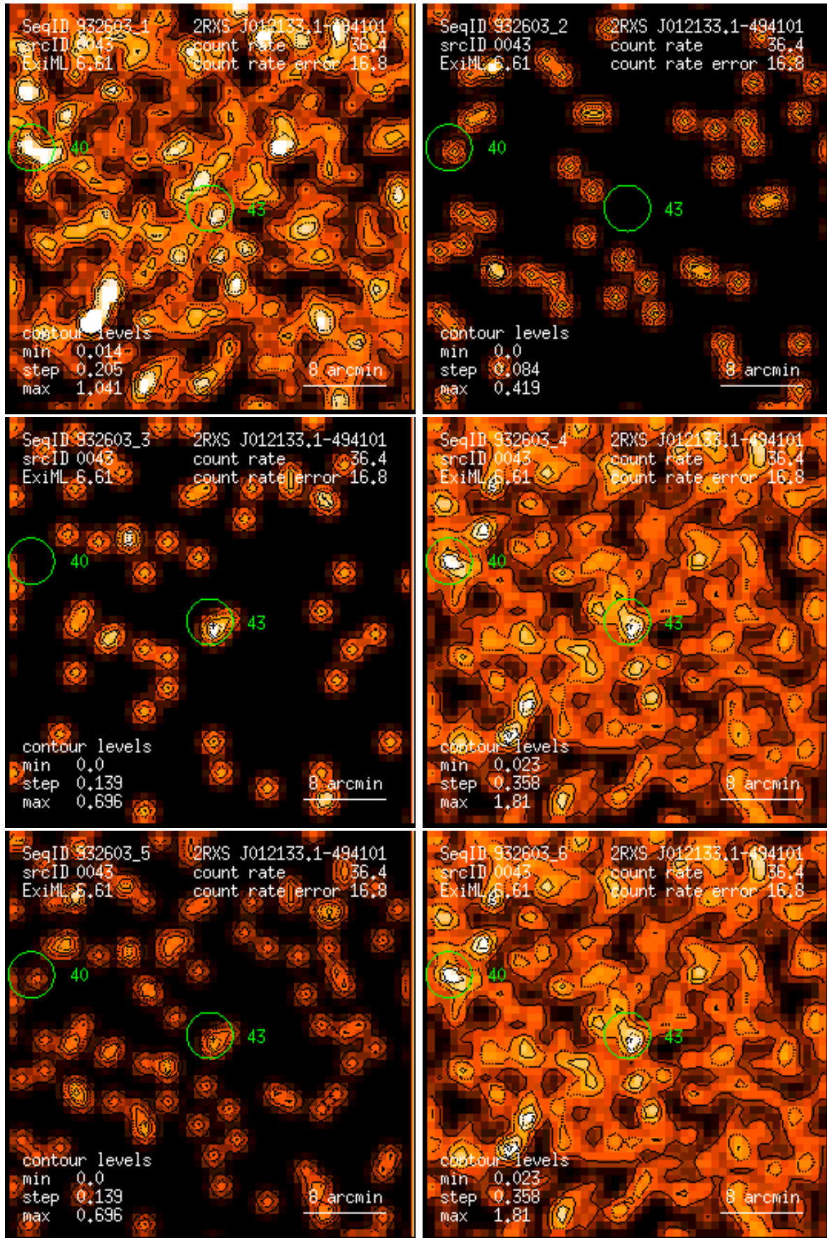
Figure 43: RASS 932603: detection 0043: band rate images, Gaussian filter: (1) PSPC channels 11 – 41, (2) 52 – 90, (3) 91 – 201, (4) 11 – 235, (5) 52 – 201, (6) 11 – 201. Broad band rates in counts/ks. Band rate contour levels in counts/ks/arcmin 2 .
