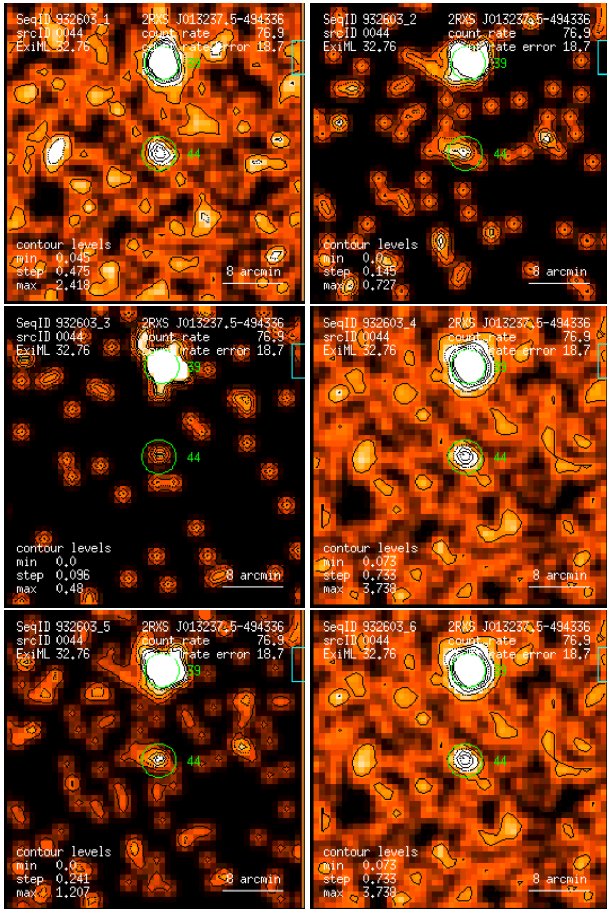
Figure 44: RASS 932603: detection 0044: band rate images, Gaussian filter: (1) PSPC channels 11 – 41, (2) 52 – 90, (3) 91 – 201, (4) 11 – 235, (5) 52 – 201, (6) 11 – 201. Broad band rates in counts/ks. Band rate contour levels in counts/ks/arcmin 2 .
