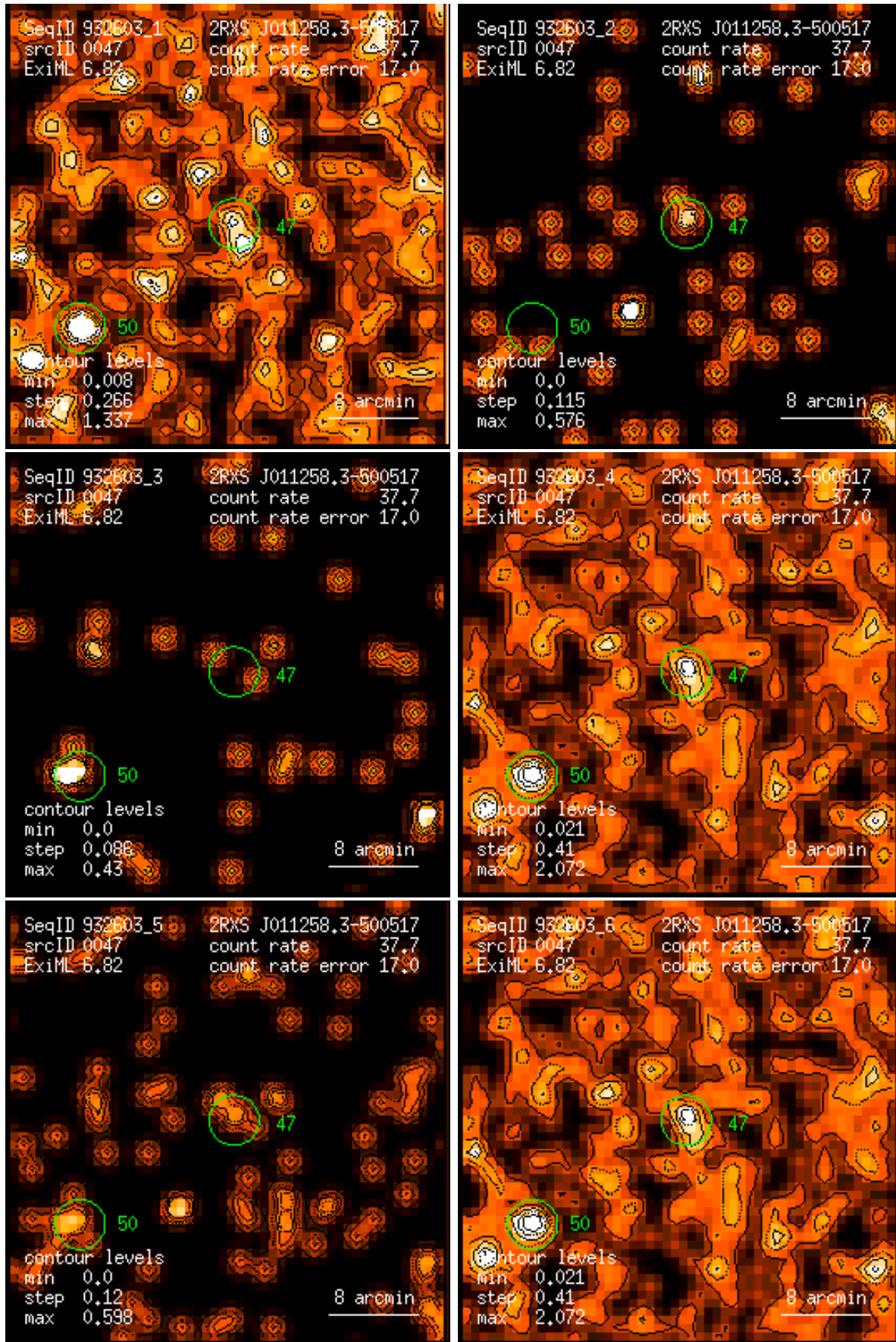
Figure 47: RASS 932603: detection 0047: band rate images, Gaussian filter: (1) PSPC channels 11 – 41, (2) 52 – 90, (3) 91 – 201, (4) 11 – 235, (5) 52 – 201, (6) 11 – 201. Broad band rates in counts/ks. Band rate contour levels in counts/ks/arcmin 2 .
