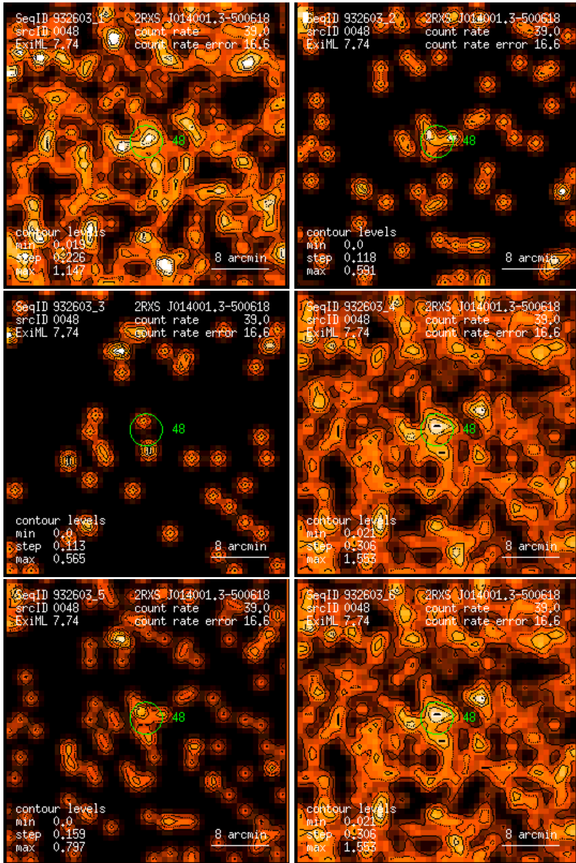
Figure 48: RASS 932603: detection 0048: band rate images, Gaussian filter: (1) PSPC channels 11 – 41, (2) 52 – 90, (3) 91 – 201, (4) 11 – 235, (5) 52 – 201, (6) 11 – 201. Broad band rates in counts/ks. Band rate contour levels in counts/ks/arcmin 2 .
