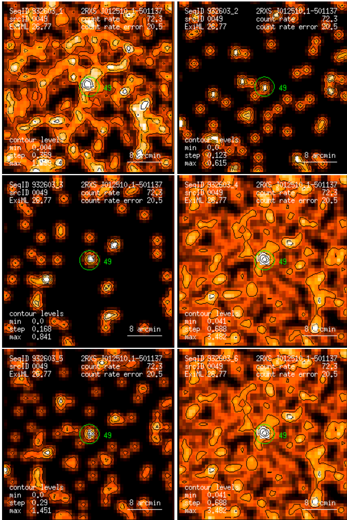
Figure 49: RASS 932603: detection 0049: band rate images, Gaussian filter: (1) PSPC channels 11 – 41, (2) 52 – 90, (3) 91 – 201, (4) 11 – 235, (5) 52 – 201, (6) 11 – 201. Broad band rates in counts/ks. Band rate contour levels in counts/ks/arcmin 2 .
