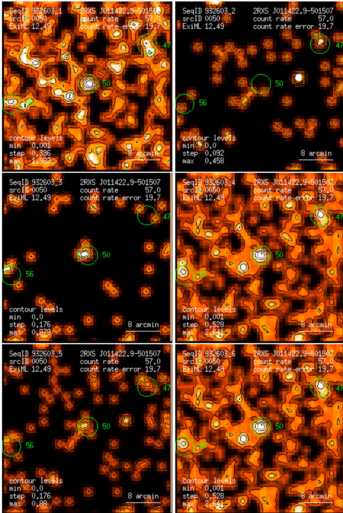
Figure 50: RASS 932603: detection 0050: band rate images, Gaussian filter: (1) PSPC channels 11 – 41, (2) 52 – 90, (3) 91 – 201, (4) 11 – 235, (5) 52 – 201, (6) 11 – 201. Broad band rates in counts/ks. Band rate contour levels in counts/ks/arcmin 2 .
