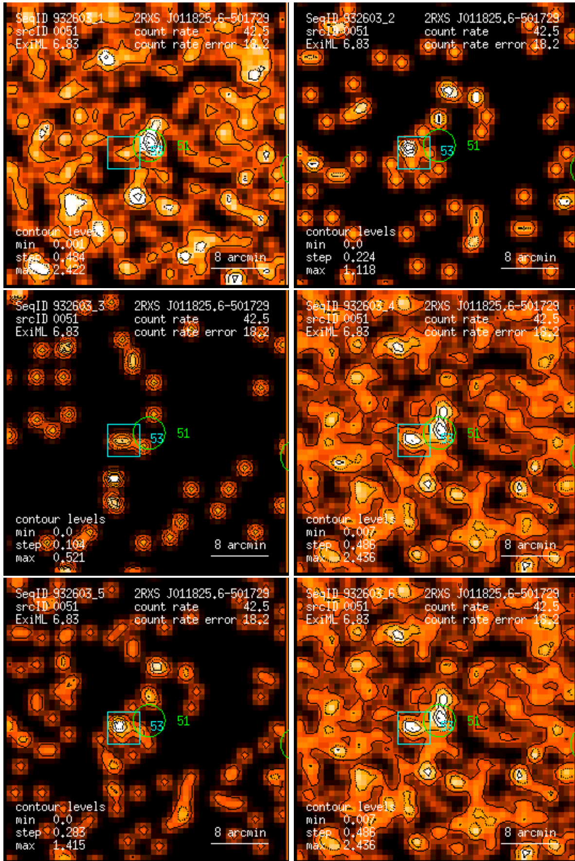
Figure 51: RASS 932603: detection 0051: band rate images, Gaussian filter: (1) PSPC channels 11 – 41, (2) 52 – 90, (3) 91 – 201, (4) 11 – 235, (5) 52 – 201, (6) 11 – 201. Broad band rates in counts/ks. Band rate contour levels in counts/ks/arcmin 2 .
