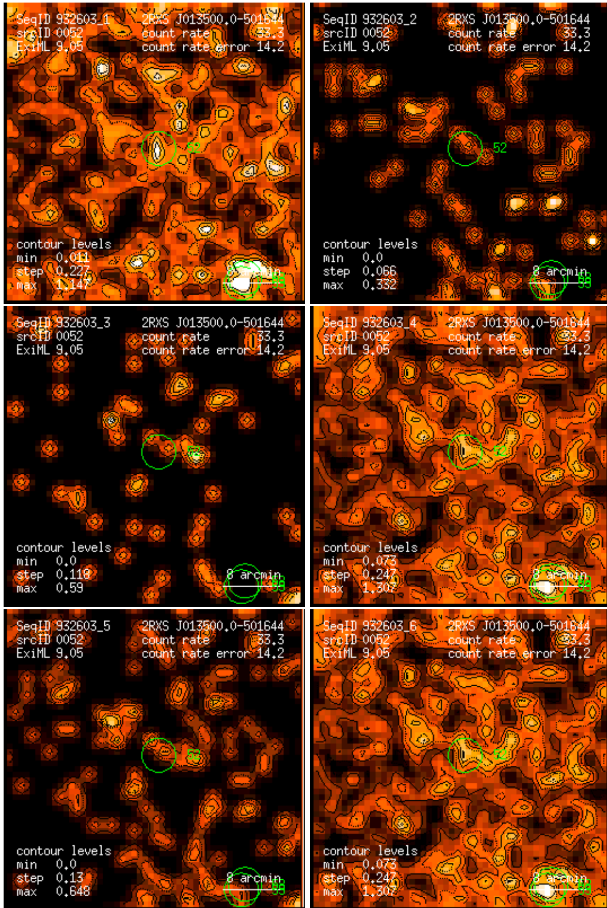
Figure 52: RASS 932603: detection 0052: band rate images, Gaussian filter: (1) PSPC channels 11 – 41, (2) 52 – 90, (3) 91 – 201, (4) 11 – 235, (5) 52 – 201, (6) 11 – 201. Broad band rates in counts/ks. Band rate contour levels in counts/ks/arcmin 2 .
