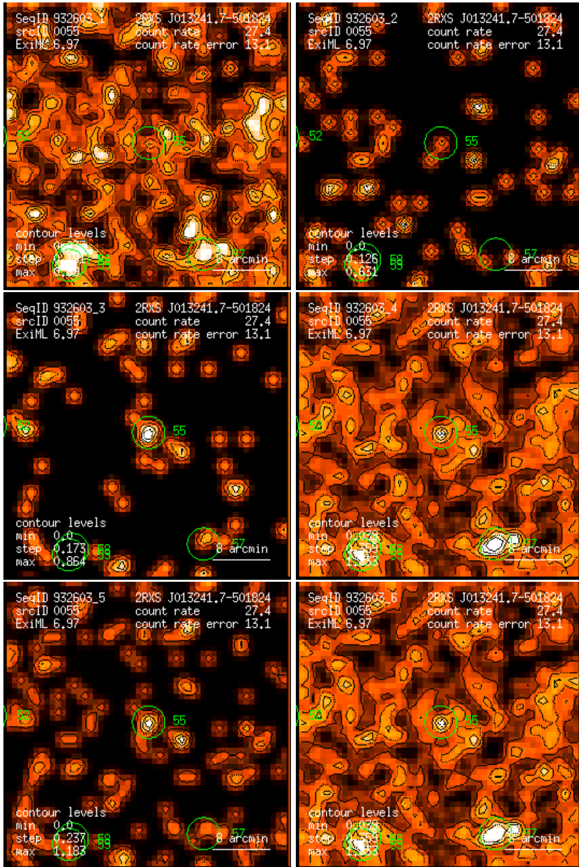
Figure 55: RASS 932603: detection 0055: band rate images, Gaussian filter: (1) PSPC channels 11 – 41, (2) 52 – 90, (3) 91 – 201, (4) 11 – 235, (5) 52 – 201, (6) 11 – 201. Broad band rates in counts/ks. Band rate contour levels in counts/ks/arcmin 2 .
