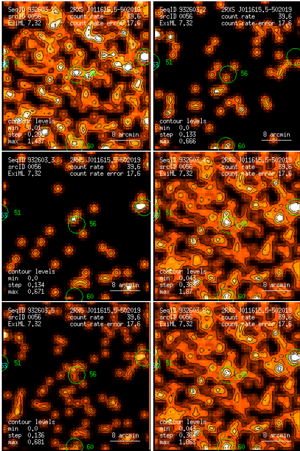
Figure 56: RASS 932603: detection 0056: band rate images, Gaussian filter: (1) PSPC channels 11 – 41, (2) 52 – 90, (3) 91 – 201, (4) 11 – 235, (5) 52 – 201, (6) 11 – 201. Broad band rates in counts/ks. Band rate contour levels in counts/ks/arcmin 2 .
