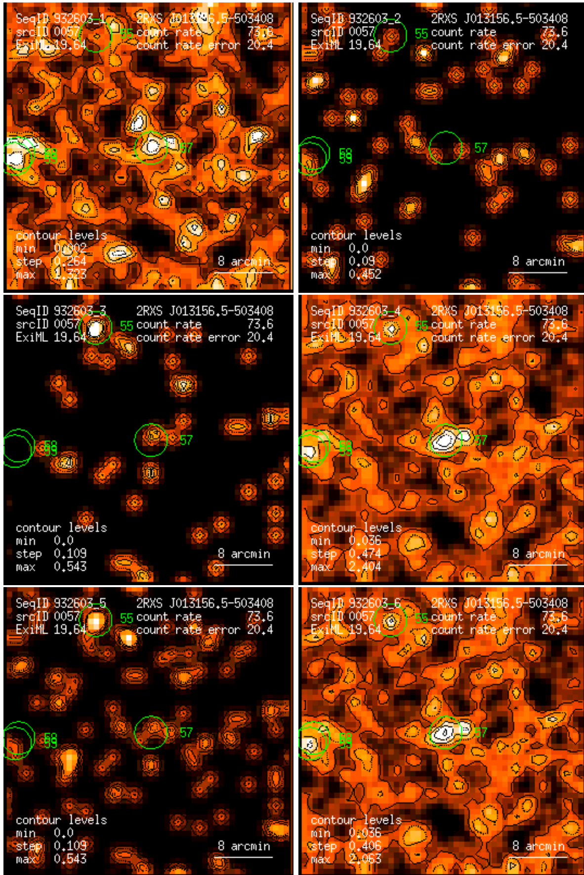
Figure 57: RASS 932603: detection 0057: band rate images, Gaussian filter: (1) PSPC channels 11 – 41, (2) 52 – 90, (3) 91 – 201, (4) 11 – 235, (5) 52 – 201, (6) 11 – 201. Broad band rates in counts/ks. Band rate contour levels in counts/ks/arcmin 2 .
