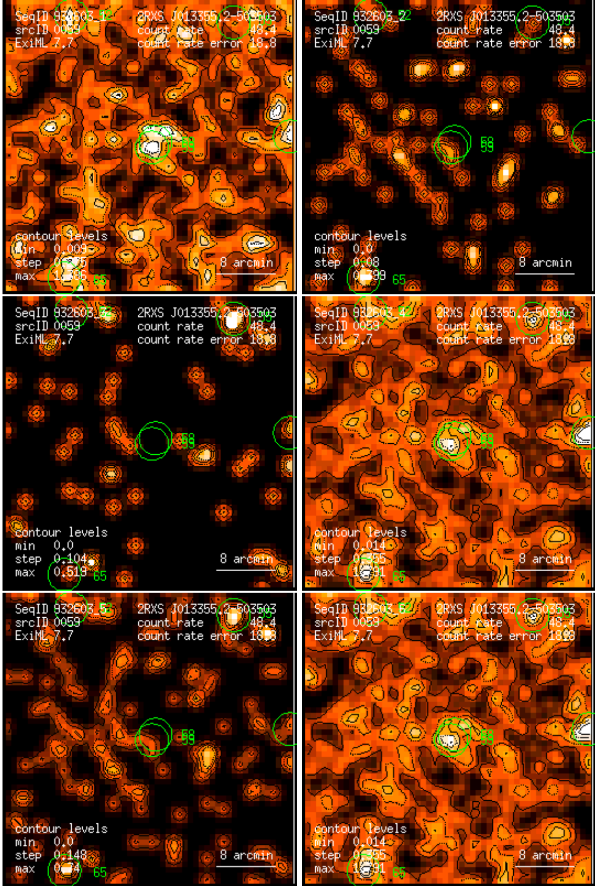
Figure 59: RASS 932603: detection 0059: band rate images, Gaussian filter: (1) PSPC channels 11 – 41, (2) 52 – 90, (3) 91 – 201, (4) 11 – 235, (5) 52 – 201, (6) 11 – 201. Broad band rates in counts/ks. Band rate contour levels in counts/ks/arcmin 2 .
