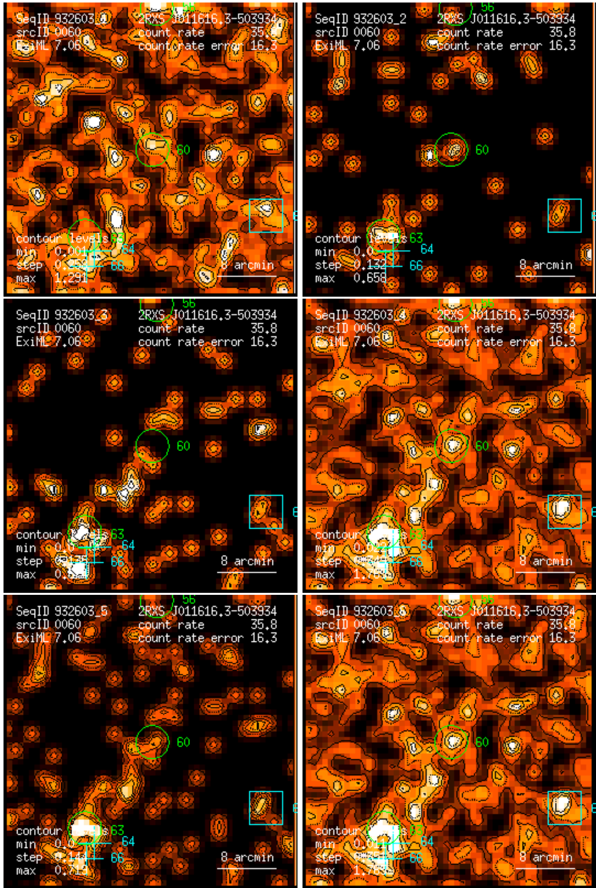
Figure 60: RASS 932603: detection 0060: band rate images, Gaussian filter: (1) PSPC channels 11 – 41, (2) 52 – 90, (3) 91 – 201, (4) 11 – 235, (5) 52 – 201, (6) 11 – 201. Broad band rates in counts/ks. Band rate contour levels in counts/ks/arcmin 2 .
