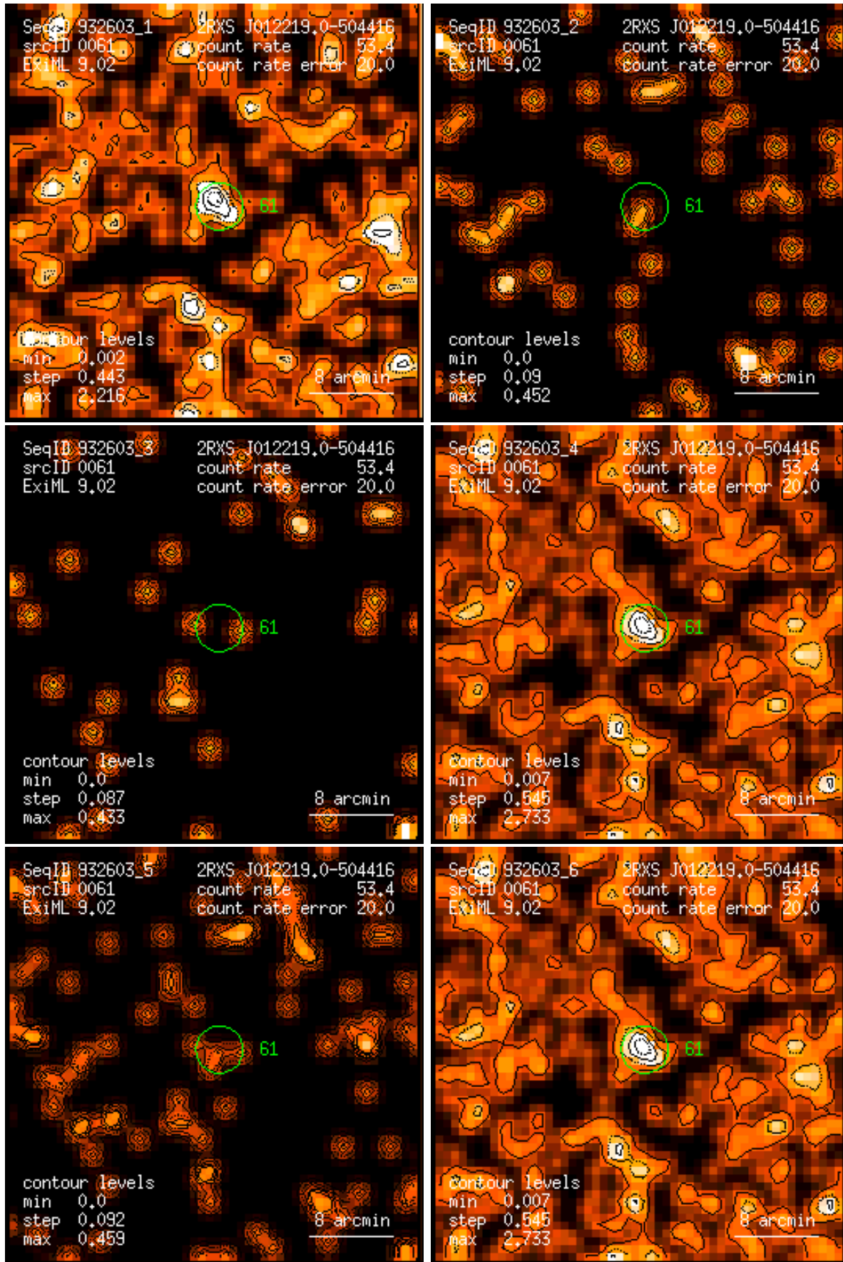
Figure 61: RASS 932603: detection 0061: band rate images, Gaussian filter: (1) PSPC channels 11 – 41, (2) 52 – 90, (3) 91 – 201, (4) 11 – 235, (5) 52 – 201, (6) 11 – 201. Broad band rates in counts/ks. Band rate contour levels in counts/ks/arcmin 2 .
