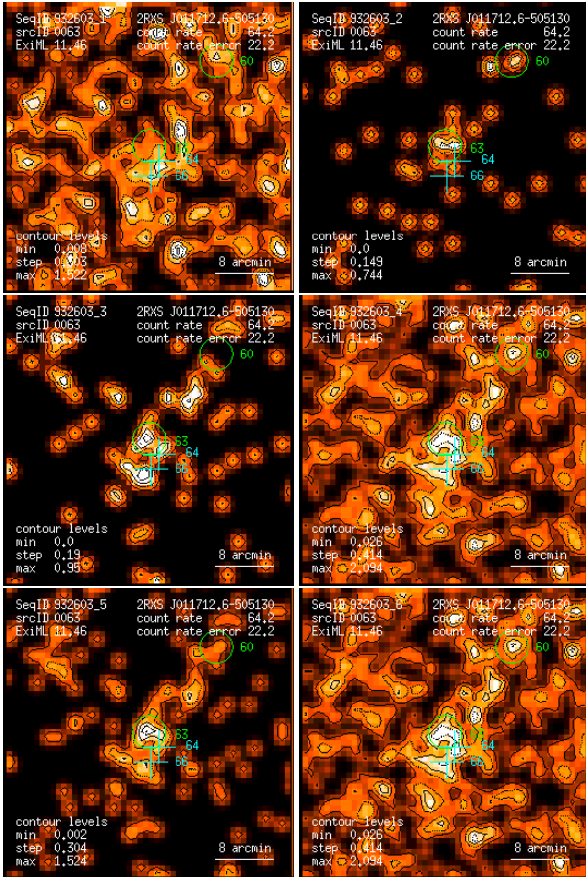
Figure 63: RASS 932603: detection 0063: band rate images, Gaussian filter: (1) PSPC channels 11 – 41, (2) 52 – 90, (3) 91 – 201, (4) 11 – 235, (5) 52 – 201, (6) 11 – 201. Broad band rates in counts/ks. Band rate contour levels in counts/ks/arcmin 2 .
