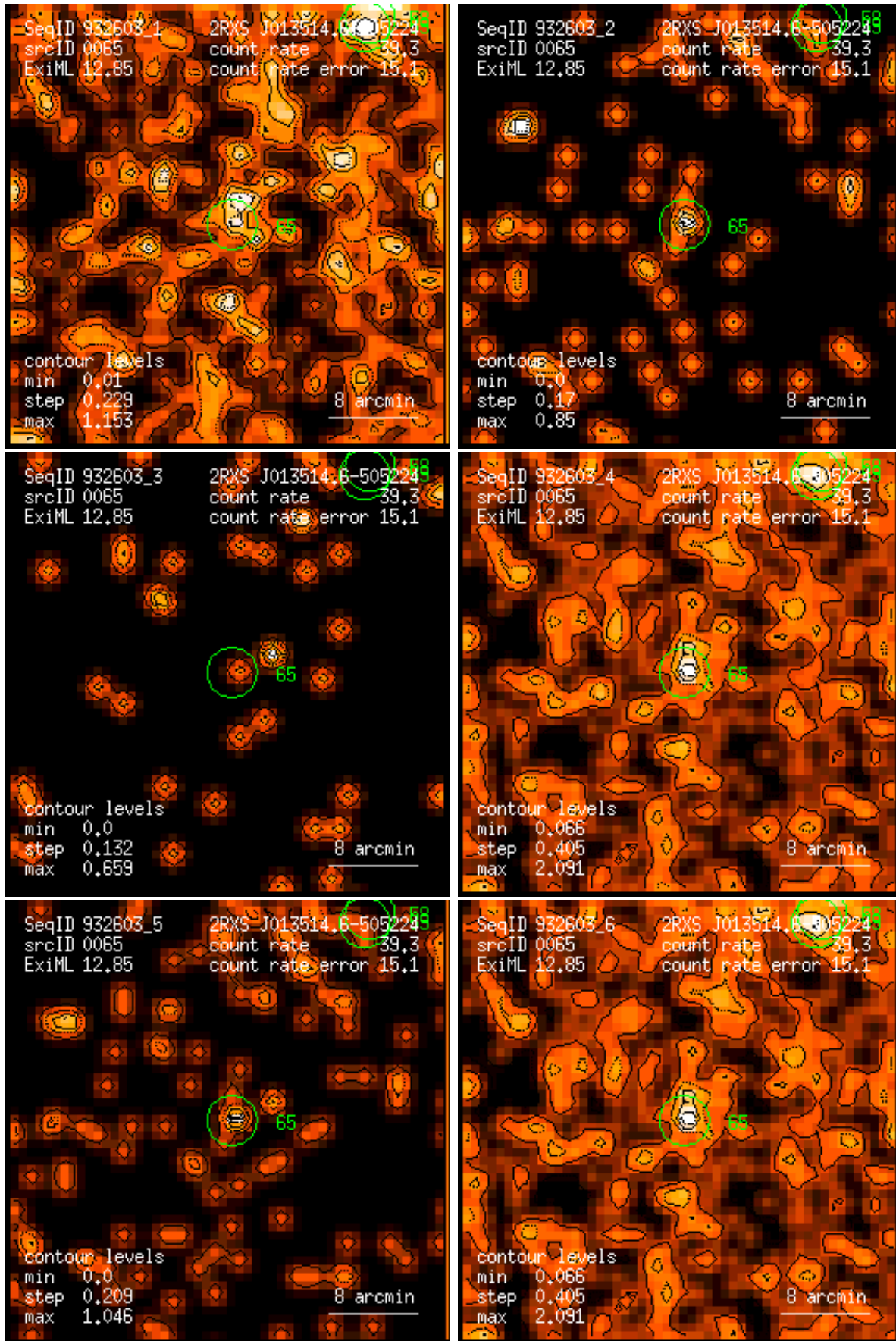
Figure 65: RASS 932603: detection 0065: band rate images, Gaussian filter: (1) PSPC channels 11 – 41, (2) 52 – 90, (3) 91 – 201, (4) 11 – 235, (5) 52 – 201, (6) 11 – 201. Broad band rates in counts/ks. Band rate contour levels in counts/ks/arcmin 2 .
