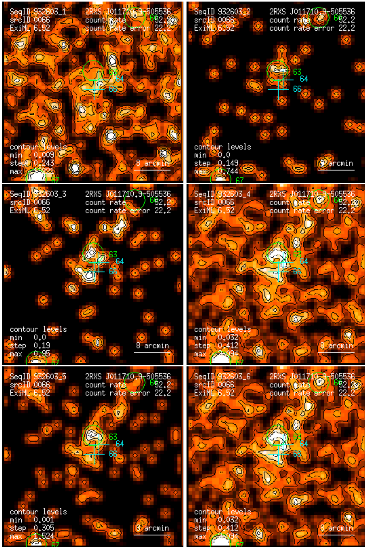
Figure 66: RASS 932603: detection 0066: band rate images, Gaussian filter: (1) PSPC channels 11 – 41, (2) 52 – 90, (3) 91 – 201, (4) 11 – 235, (5) 52 – 201, (6) 11 – 201. Broad band rates in counts/ks. Band rate contour levels in counts/ks/arcmin 2 .
