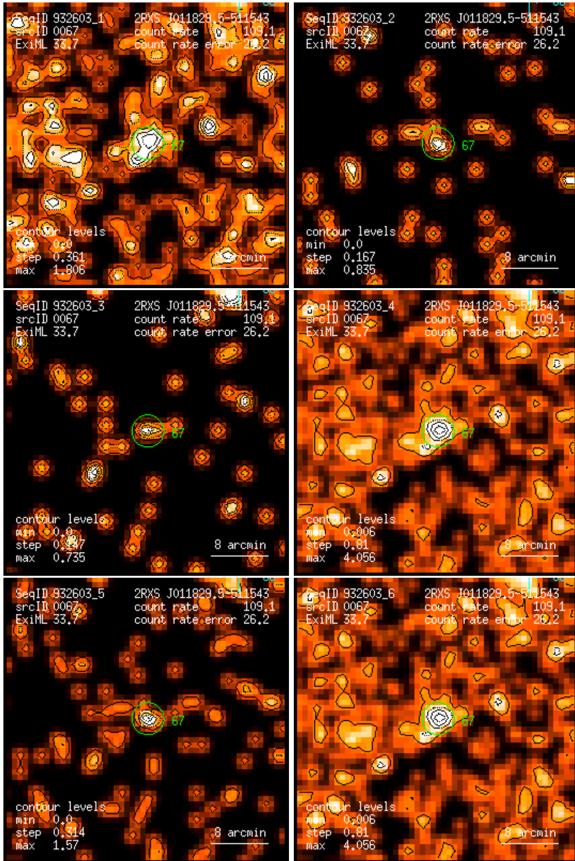
Figure 67: RASS 932603: detection 0067: band rate images, Gaussian filter: (1) PSPC channels 11 – 41, (2) 52 – 90, (3) 91 – 201, (4) 11 – 235, (5) 52 – 201, (6) 11 – 201. Broad band rates in counts/ks. Band rate contour levels in counts/ks/arcmin 2 .
