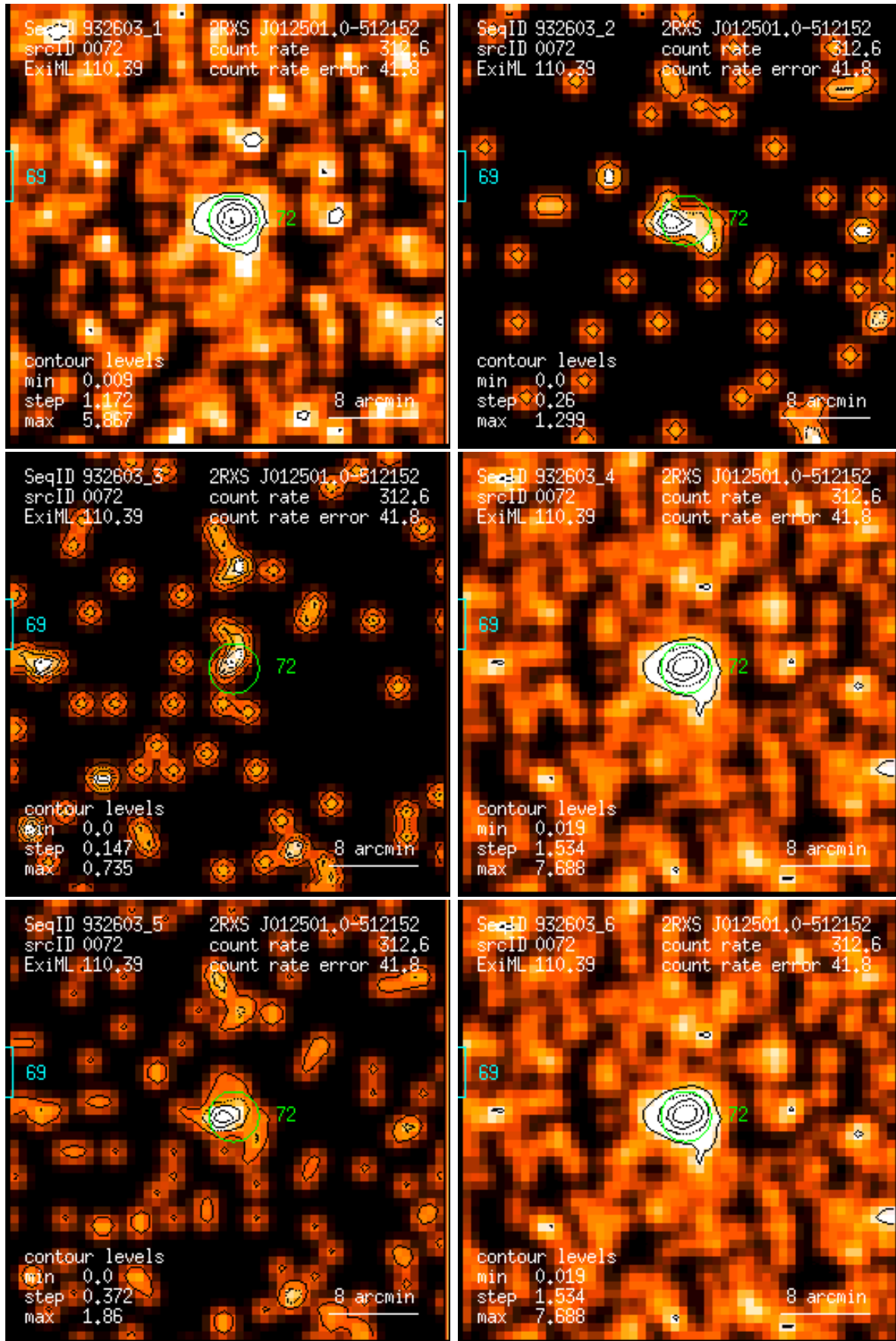
Figure 72: RASS 932603: detection 0072: band rate images, Gaussian filter: (1) PSPC channels 11 – 41, (2) 52 – 90, (3) 91 – 201, (4) 11 – 235, (5) 52 – 201, (6) 11 – 201. Broad band rates in counts/ks. Band rate contour levels in counts/ks/arcmin 2 .
