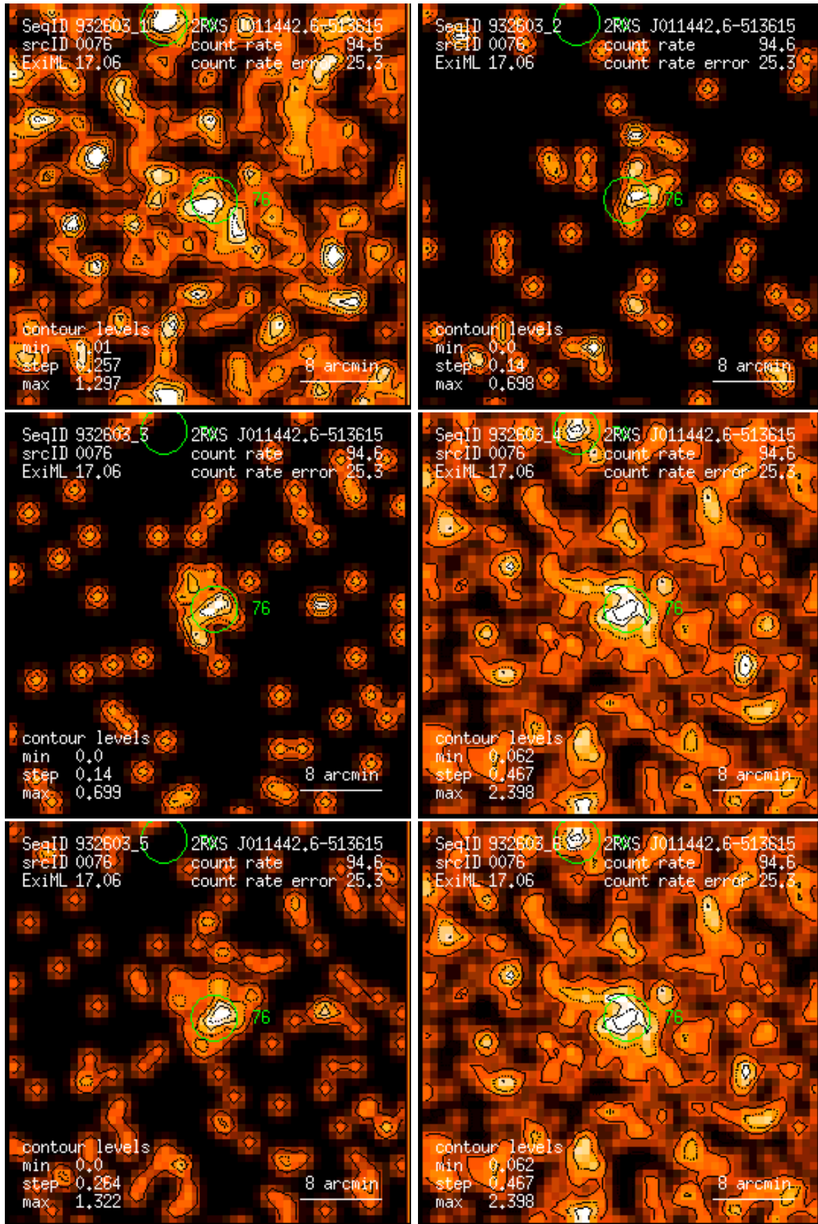
Figure 76: RASS 932603: detection 0076: band rate images, Gaussian filter: (1) PSPC channels 11 – 41, (2) 52 – 90, (3) 91 – 201, (4) 11 – 235, (5) 52 – 201, (6) 11 – 201. Broad band rates in counts/ks. Band rate contour levels in counts/ks/arcmin 2 .
