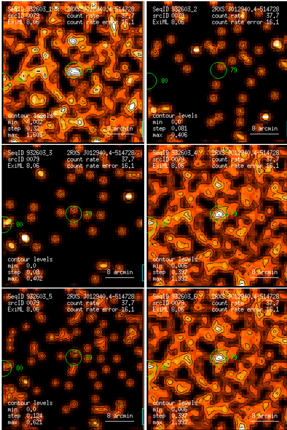
Figure 79: RASS 932603: detection 0079: band rate images, Gaussian filter: (1) PSPC channels 11 – 41, (2) 52 – 90, (3) 91 – 201, (4) 11 – 235, (5) 52 – 201, (6) 11 – 201. Broad band rates in counts/ks. Band rate contour levels in counts/ks/arcmin 2 .
