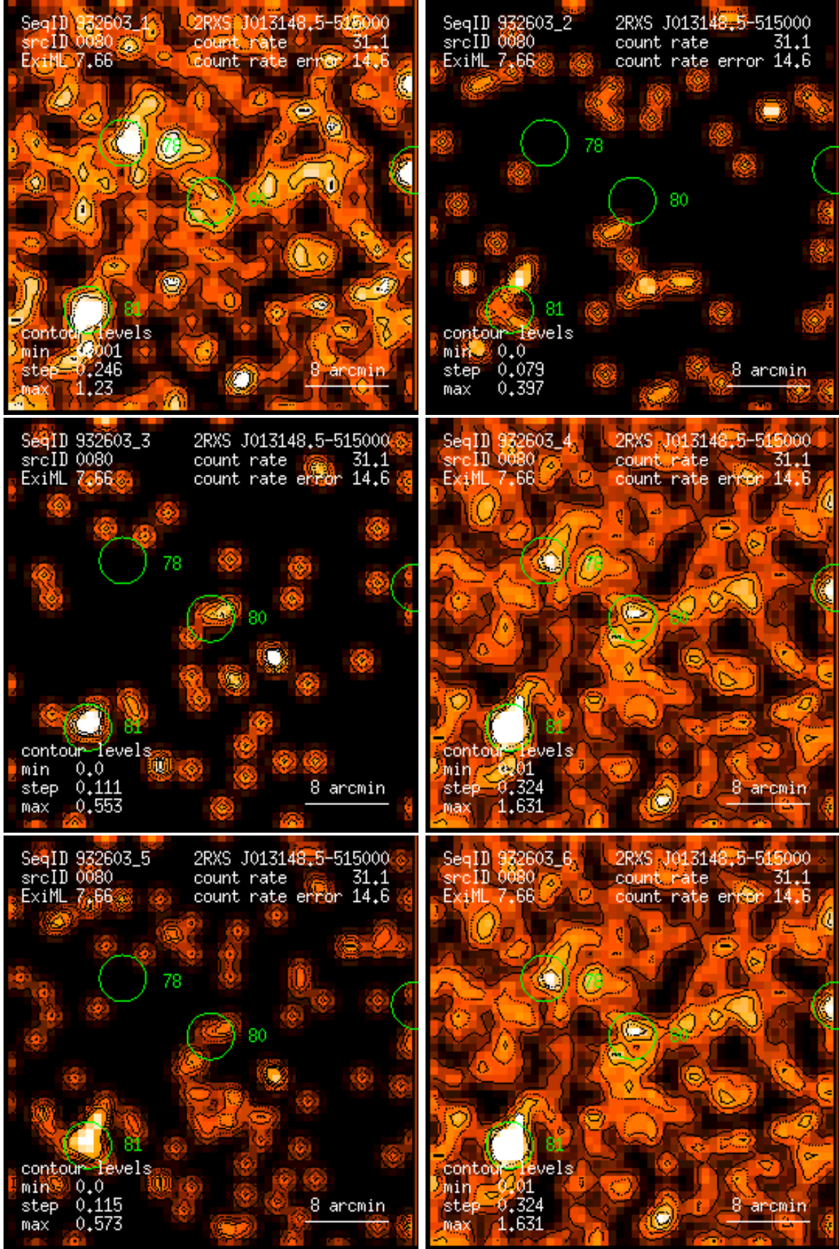
Figure 80: RASS 932603: detection 0080: band rate images, Gaussian filter: (1) PSPC channels 11 – 41, (2) 52 – 90, (3) 91 – 201, (4) 11 – 235, (5) 52 – 201, (6) 11 – 201. Broad band rates in counts/ks. Band rate contour levels in counts/ks/arcmin 2 .
