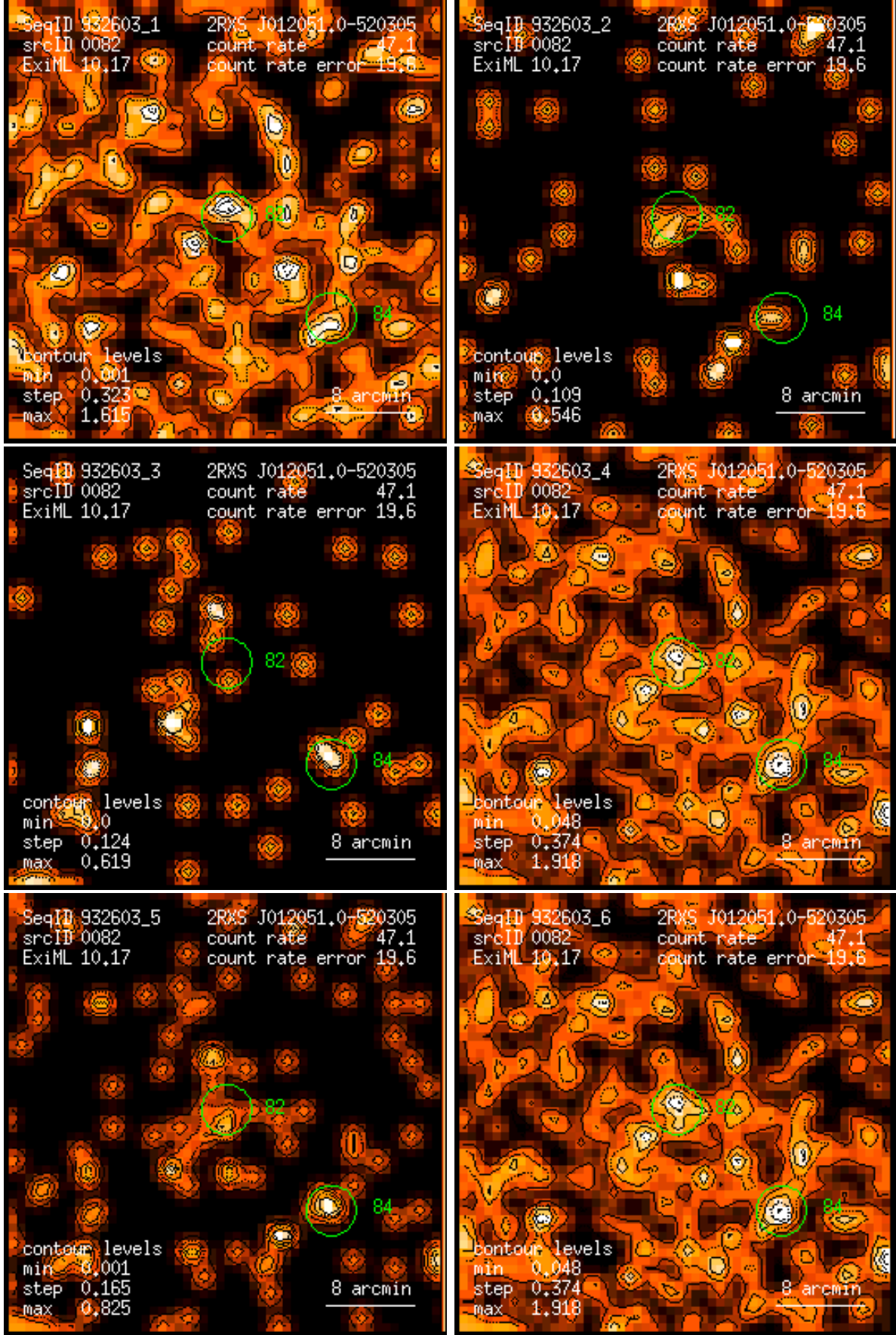
Figure 82: RASS 932603: detection 0082: band rate images, Gaussian filter: (1) PSPC channels 11 – 41, (2) 52 – 90, (3) 91 – 201, (4) 11 – 235, (5) 52 – 201, (6) 11 – 201. Broad band rates in counts/ks. Band rate contour levels in counts/ks/arcmin 2 .
