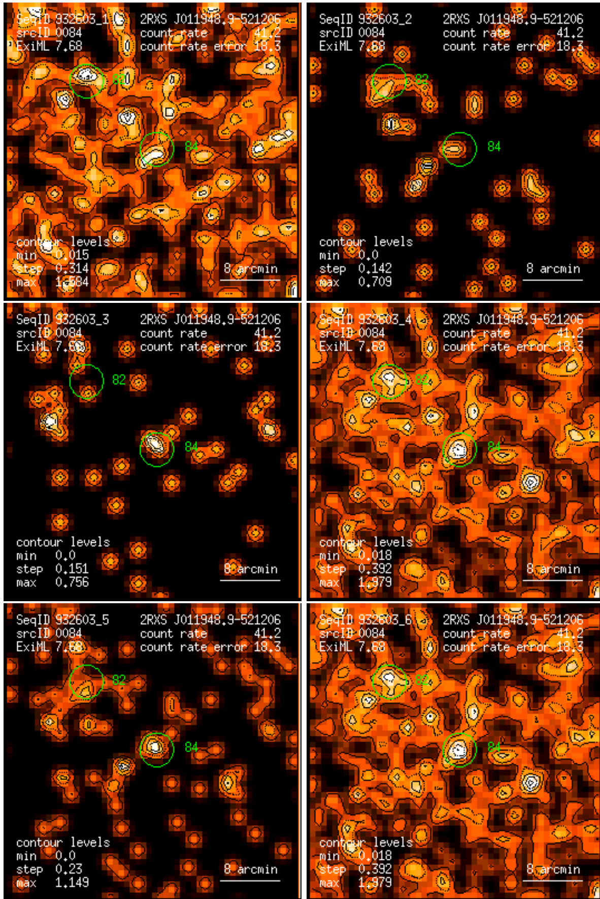
Figure 84: RASS 932603: detection 0084: band rate images, Gaussian filter: (1) PSPC channels 11 – 41, (2) 52 – 90, (3) 91 – 201, (4) 11 – 235, (5) 52 – 201, (6) 11 – 201. Broad band rates in counts/ks. Band rate contour levels in counts/ks/arcmin 2 .
