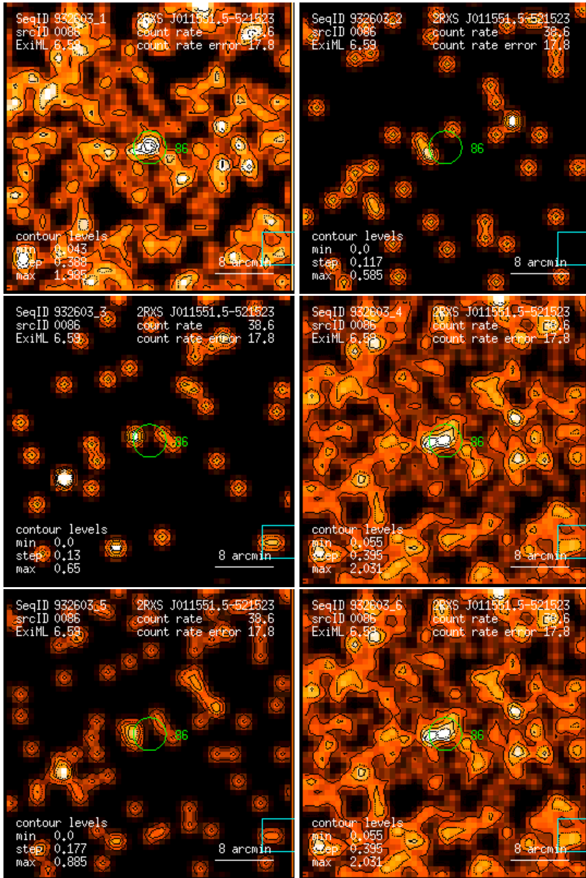
Figure 86: RASS 932603: detection 0086: band rate images, Gaussian filter: (1) PSPC channels 11 – 41, (2) 52 – 90, (3) 91 – 201, (4) 11 – 235, (5) 52 – 201, (6) 11 – 201. Broad band rates in counts/ks. Band rate contour levels in counts/ks/arcmin 2 .
