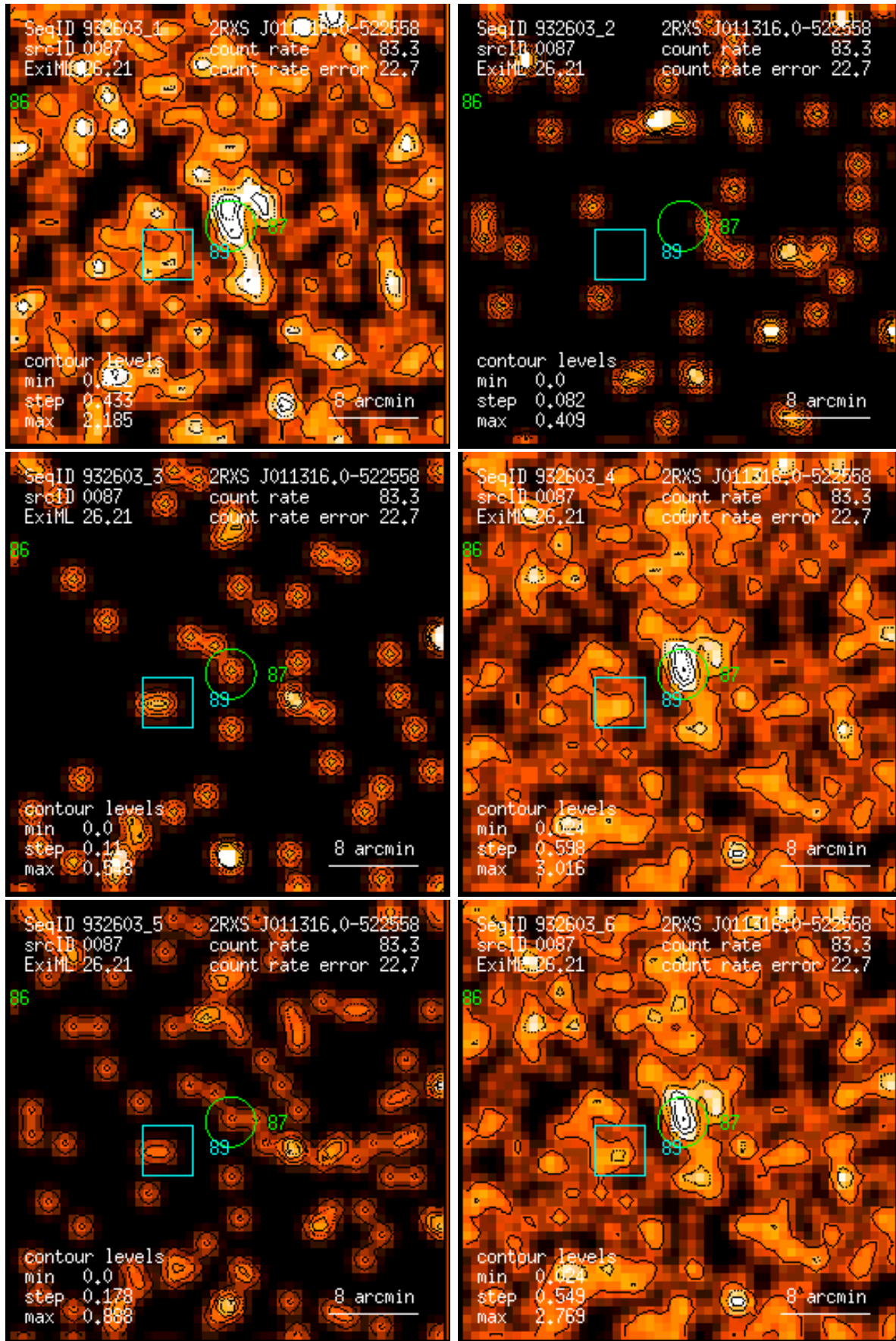
Figure 87: RASS 932603: detection 0087: band rate images, Gaussian filter: (1) PSPC channels 11 – 41, (2) 52 – 90, (3) 91 – 201, (4) 11 – 235, (5) 52 – 201, (6) 11 – 201. Broad band rates in counts/ks. Band rate contour levels in counts/ks/arcmin 2 .
