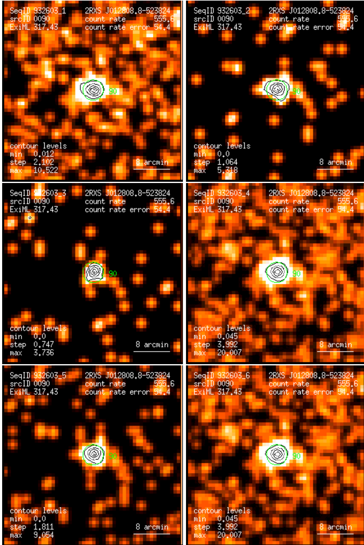
Figure 90: RASS 932603: detection 0090: band rate images, Gaussian filter: (1) PSPC channels 11 – 41, (2) 52 – 90, (3) 91 – 201, (4) 11 – 235, (5) 52 – 201, (6) 11 – 201. Broad band rates in counts/ks. Band rate contour levels in counts/ks/arcmin 2 .
